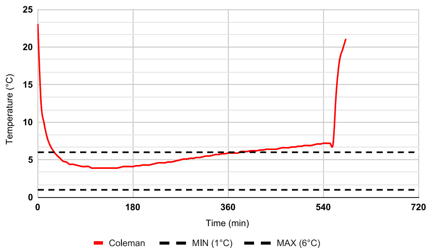
FIGURE 2 Representative temperature log for performance validation. Initial temperatures were above 6^{\circ}\text{C} as the cooler and data logger were not conditioned at refrigerator temperatures. End of storage excursion at 378 min.
