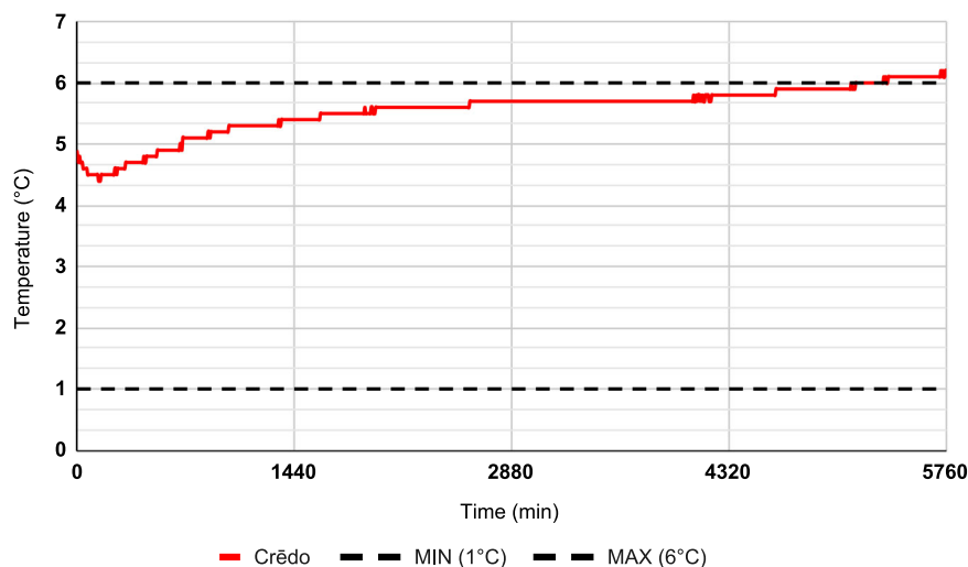
FIGURE 3 Representative temperature log for the ProMed validation. Temperature excursion at 5340 min.
