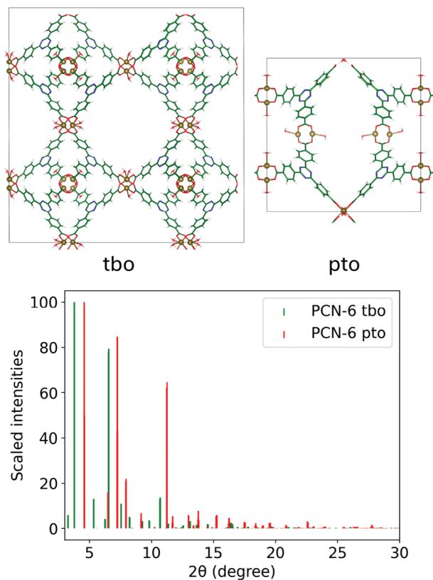
Figure 4. PCN-6' structures with topologies tbo and pto optimized at DFT level with PBE-D3BJ functional [38,39] (top); and related computational PXRD pattern (bottom). Colorcode: Cu gold, N blue, O red, C green, H white.
