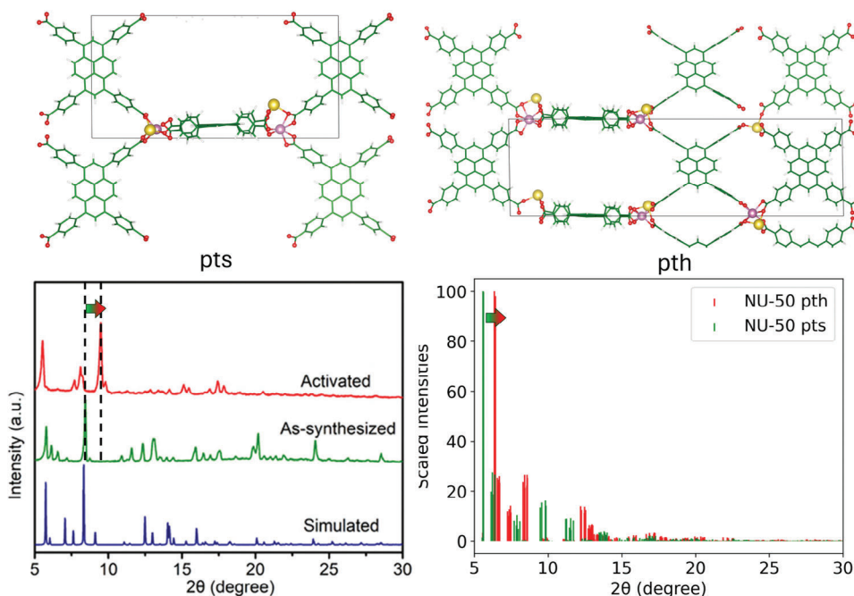
Figure 5. NU-50 structures with topologies pts and pth optimized at DFT level with PBE-D3BJ functional [38,39] (top); related computational PXRD pattern (bottom right) showing the peak shift with potential relation to post-activated structure deformation; and experimental PXRD pattern (bottom left) from reference [34] added for comparison. Colorcode: In pink, Na yellow, O red, C green, H white.
