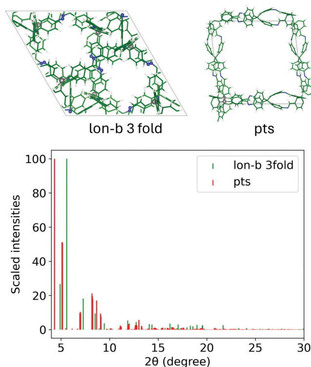
Figure 6. COF LZU-111 structures with topologies lon-b threefold interpenetrated, and pts optimized at DFT level with r^2 SCAN+rVV10 functional [41,42] (top), and related computational PXRD pattern (bottom) showing for comparison. Colorcode: Si gray, N blue, O red, C green, H white.
