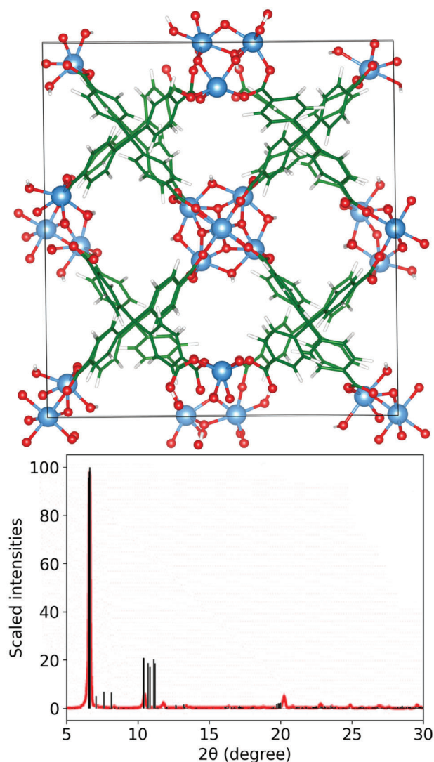
Figure 3. MOF-841 in topology flu optimized at DFT level with PBE-D3BJ functional. [38,39] Experimental PXRD pattern (red line) taken from previously published data from reference. [31] Computational PXRD pattern calculated in this work (black lines). Colorcode: Zr blue, O red, C green, H white.
