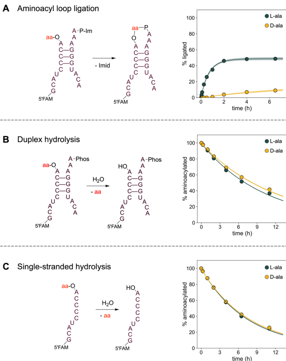
Figure 1. Reaction Schemes and Time Courses for aminoacyl-RNA loop-closing ligation and hydrolysis. (A) Left: reaction scheme for aminoacyl-RNA loop-closing ligation using an imidazole-activated capture strand. Right: time course of the ligation reaction. (B, C) Left: reaction schemes for aminoacyl-RNA hydrolysis under duplex and single-stranded conditions. Right: time courses of the hydrolysis reaction. Reaction rates are presented in Tables 1, S1 and S2, and gel images are shown in Figure S1. All reactions were conducted at 0 °C in 5 mM MgCl 2 , 100 μM Na 2 EDTA, 100 mM imidazole, pH 8.0, and 5 μM RNA oligonucleotides. Shaded regions envelope the 95% prediction interval as determined from the kinetic model.
