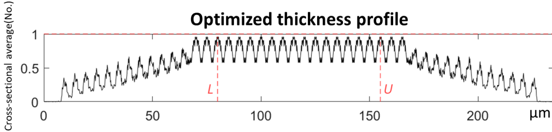
Figure S5. The optimized average thickness profile of the \text{MoS}_2 channel with n^* = 27 single pass parallel lines (i.e., Figure 3a) abreast, spaced by d^* = 5 \mu m . The center part of our interest is between two vertical dashed lines, each of which represents L and U , respectively. We used C = 70 . The horizontal dashed red line represents T = 1 .
