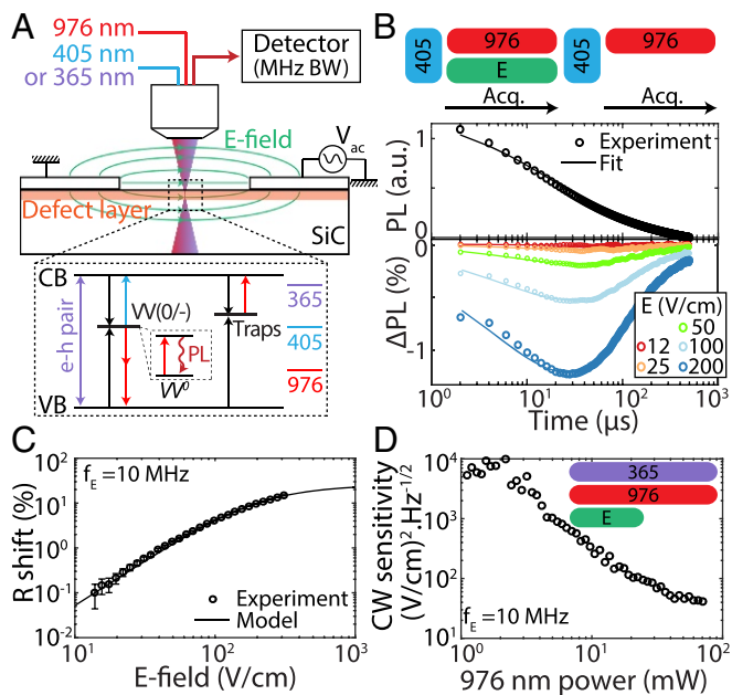
Fig. 1. EOC. (A) Schematic of the optical setup with one reset color (365 nm or 405 nm) and one pump color (976 nm). Illumination at 365 nm generates electron-hole (e-h) pairs that reset VV to VV 0 (bright state) in the steady state, at 405 nm directly ionizes VV - (dark state) to VV 0 , and at 976 nm excitation converts VV 0 to VV - by direct two-photon ionization or indirectly by one-photon ionization of local traps (11, 18). In addition, VV 0 photoluminescence is provided through excitation at 976 nm. VV(0/-) is the transition energy level between the neutral and negatively charged states. VB and CB are the valence and conduction bands, respectively. An RF electric field (rms amplitude E , frequency f_E ) is applied across a coplanar capacitor with a 17- \mu\text{m} gap. VVs are created by carbon implantation immediately below the surface. A fast detector with 10-MHz bandwidth (BW) allows for direct detection of a full OCC transient signal in a single measurement. (B) VV is first reset to its bright state (VV 0 ) by 405-nm illumination, followed by PL detection (Top) of the charge conversion toward the VV dark state by 976-nm excitation. Bottom shows the difference between conversion with and without applied electric field (10 MHz). Data are fitted to a stretched exponential function with R = 42 kHz and n = 0.54 obtained using a global fit for all electric field values. (C) Fitted decay rate shifts as a function of electric field. Error bars are 95% confidence intervals. (D) EOC sensitivity with continuous (CW) laser (365 nm and 976 nm) pumping as a function of 976-nm laser power. We estimate a 10% error in electric field estimation, corresponding to 20% error in sensitivity (not shown). Acq., acquisition.
