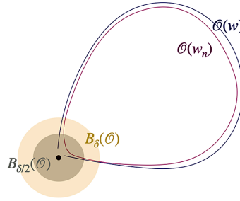
FIGURE 1. Proof of Proposition 3.9. The closed orbit \mathcal{O} is schematically represented by the black dot.
