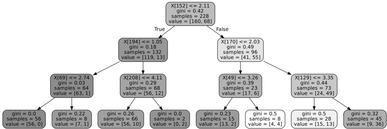
eFigure. One of Two Decision Trees for a Test in the CAD-PTSD (Exemplar)
