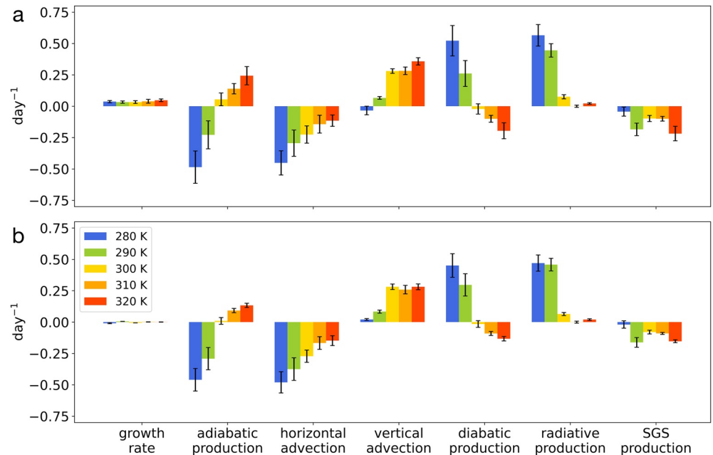
Figure 2. The LMSE variance analysis for 2D control experiments (Equation 4). The upper panel shows the budget averaged in the development stage, and the lower panel shows that averaged in the maintenance stage. The error bars show uncertainty by using different window lengths of temporal and spatial running averages (varying from 1 day to 10 days, from 40 to 120 km) to get large-scale perturbations and using different window lengths (varying from 5, 10, 15, 20, to 25 days) to average the LMSE budget in the development and maintenance stages. The “adiabatic production” represents the total contribution from horizontal and vertical advection processes. The “diabatic production” represents the total contribution from radiation and SGS processes.
