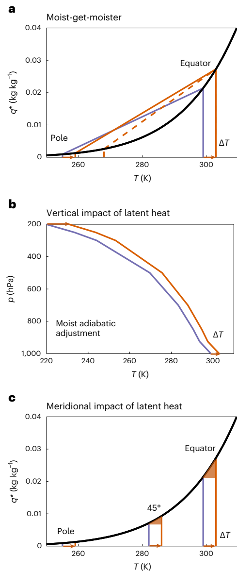
Fig. 3 | Robust responses of moisture under climate change following the Clausius–Clapeyron relation. a , Moist-get-moister response involves warmer air ‘holding’ more moisture following the Clausius–Clapeyron relation (black line), with the largest increase near the Equator. It implies an increased meridional gradient of saturation specific humidity under uniform warming (slopes of blue versus orange lines) and polar-amplified warming (compare y-axis range of solid blue and dashed orange lines). b , Latent heat release aloft by rising air parcels that ‘hold’ more moisture following moist adiabatic adjustment under climate change (uniform surface warming indicated from blue to orange). c , The latent heat release aloft (orange triangle) is largest at the Equator following the Clausius–Clapeyron relation (black line).
