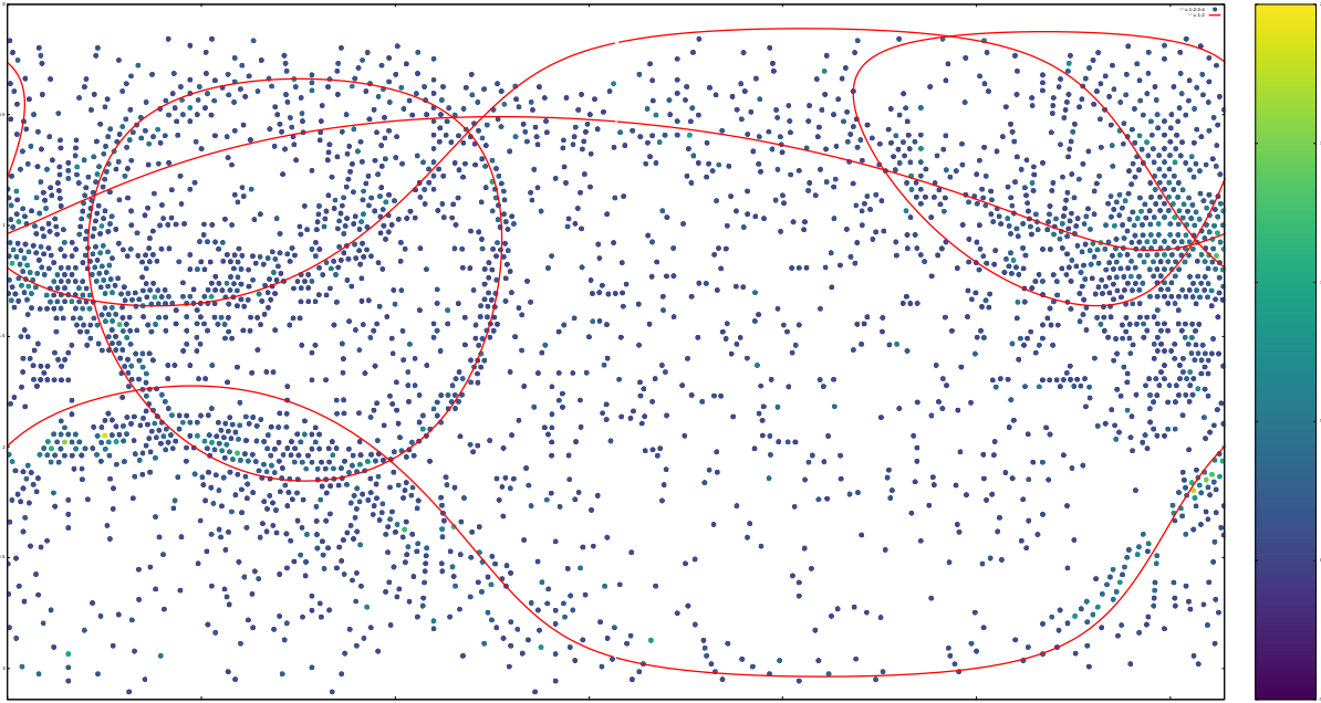
Figure 3.5: Plot showing the 5 peaks detected in an atmospheric neutrino event.
