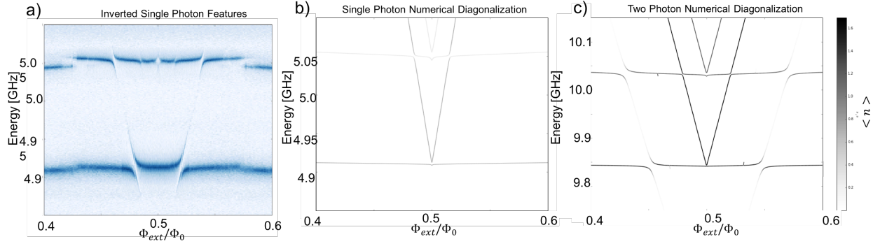
Figure 7.5: a) Experimental Data of Single Tone scan near half-flux quantum when the device is in the persistent negative temperature state. b) Expectation value of the photon number for the Eigen solution of the coupled Hamiltonian, showing a different energy spectrum than what was measured. c) Expectation value of a higher energy manifold for the Eigen solution of the coupled matrix. Showing the similar features of the inverted spectrum with this higher energy manifold. In figure 8.4, we see that the otherwise prevalent photon-assisted features line up in this area and may serve to excite us into this higher energy manifold.
