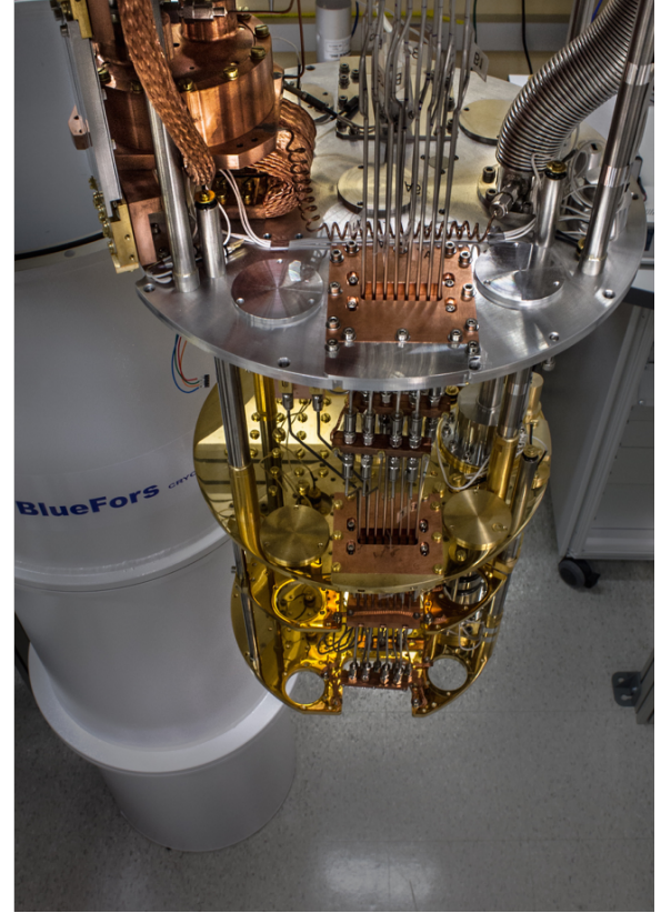
Figure 5.3: a) Wiring Diagram of heavy fluxonium setup. b) Photo of BluFors Dilution Refrigerator used to measure the device. In the photo, the RF lines can be seen in the middle and are thermalized to each stage with copper clamps, machined by myself and Andrew Oriani.
