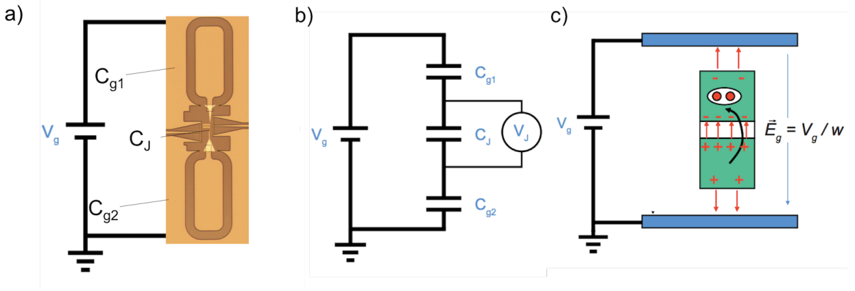
Figure 3.4: a) Image of fluxonium Sample with a cartoon voltage which arises from a photon being present inside the readout resonators (capacitively coupled, but not seen in the photo) b) A voltage divider diagram for a capacitively coupled junction with capacitance C_J c) This can be approximated as a dipole inside an electric field to gain intuition as to how state readout works.
