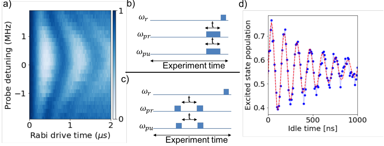
Figure 6.10: a) Demonstration of a successful Rabi oscillation with a T_\pi of \sim 440\text{nsec} , a substantial improvement in the very slow excitation seen in figure 6.9b. Here you can see the typical chevron patterns which arise from an increase rabi oscillation when driving slightly off resonance. b) A demonstration of the ‘three tone’ Raman rabi experiment. c) Demonstration of the ‘three tone’ Ramsey experiment. d) A Ramsey experiment, which allows us to directly measure the T_2 of the device.
