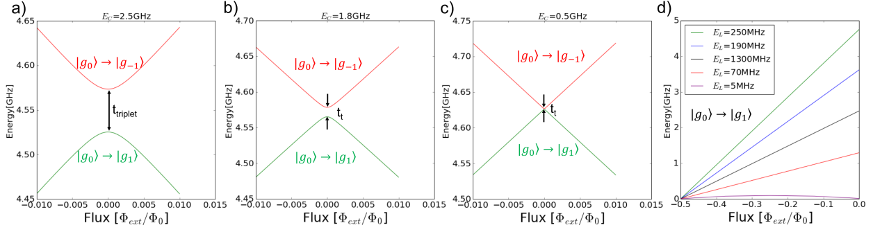
Figure 3.3: Suppression of the tunneling matrix element also comes with a loss of the sweet spot, which is ideal for a long T_2 coherence time. a-d are an increasing capacitance (the effective mass), which results in a decrease in the tunneling between |g_0\rangle and |g_1\rangle , but also the loss of a sweet spot. A tradeoff between these two factors will be important when engineering this qubit for the purpose of quantum information.
