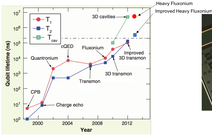
Figure 1.5: a) A chart from [9] showing the improvement of qubit lifetimes and coherences over the past couple of decades with recent results added to the chart [14, 11, 16]. It is this substantial improvement in coherence, along with the versatility of superconducting circuits that has made them the popular system to pursue a large quantum computer. Note the recent result of the heavy fluxonium [14, 11] achieving T_1 s above a millisecond and the improved heavy fluxonium [16] achieving T_2 s of several hundred microseconds and for the points measured hitting the limit of T_2 = 2 T_1 . This improvement was the result of carefully trading off the benefit of a suppressed dipole element for a good T_1 vs having a ‘sweet spot’ for good T_2 s. b) A photo of the 19-qubit quantum processor by IBM. In this photo, they use 2D transmon qubits coupled to nearest neighbors via capacitive coupling.
