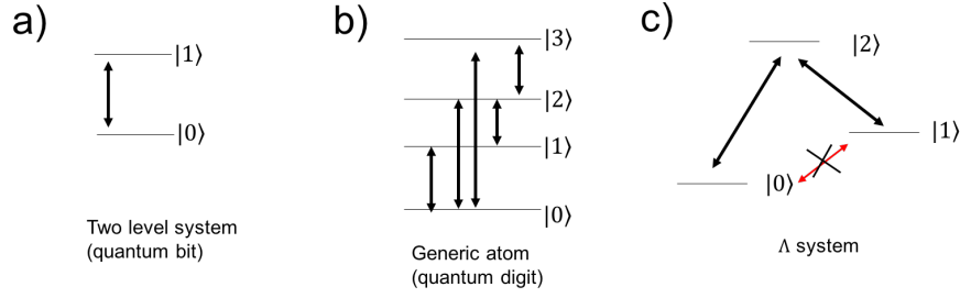
Figure 2.3: Different realizations of artificial quantum systems that are discussed in this thesis. a) A two-level system. Though the transmon is not a true two-level system, we are able to access the first two levels and study coherent oscillations between them. At low driving powers, the higher energy levels can be ignored, though it is useful to not ignore them in the case of fast-flux gates for multi-mode realization of a quantum system [17]. b) A generic atom consisting of multiple energy levels, generally known as a ‘quantum digit’ (qudit). c) A \Lambda system with two states ( |0\rangle and |1\rangle ) cannot directly couple, but their interactions can be mediated by a third higher auxiliary level ( |2\rangle ) that couples to both [14].
