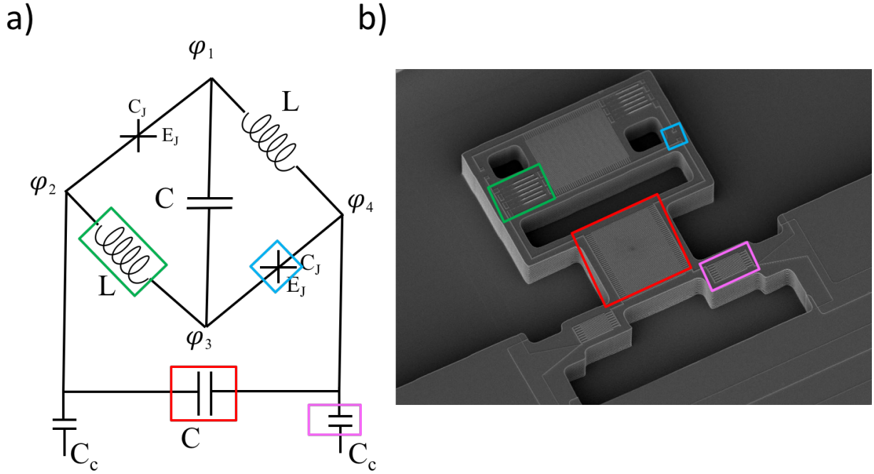
Figure 8.2: a) The circuit diagram for an asymmetrically coupled 0- \pi circuit. Colored boxes are to guide the eye for the fabrication image seen in b. b) An SEM image of process development for the 0- \pi circuit. In particular, this process was to determine the feasibility of using stacked junctions with a deep silicon etch to reduce the amount of stray capacitance contributing to C_J .
