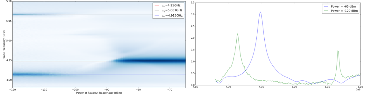
Figure 6.2: Single Tone Spectroscopy power sweep. a) A 2D plot showing the saturation of the heavy fluxonium qubit at high powers ( > -90 dB) revealing the bare resonance, \omega_r of the readout resonator. At lower powers ( < -100 dB) the qubit plasmon \omega_q and the dressed resonator, \omega_{r'} are seen, revealing the ‘plasmonic dispersive’ coupling regime. b) A line cut of the two characteristic regimes. The total area under the curve must be conserved, and the bare resonator transmission amplitude is used to normalize the spectra in all the figures.
