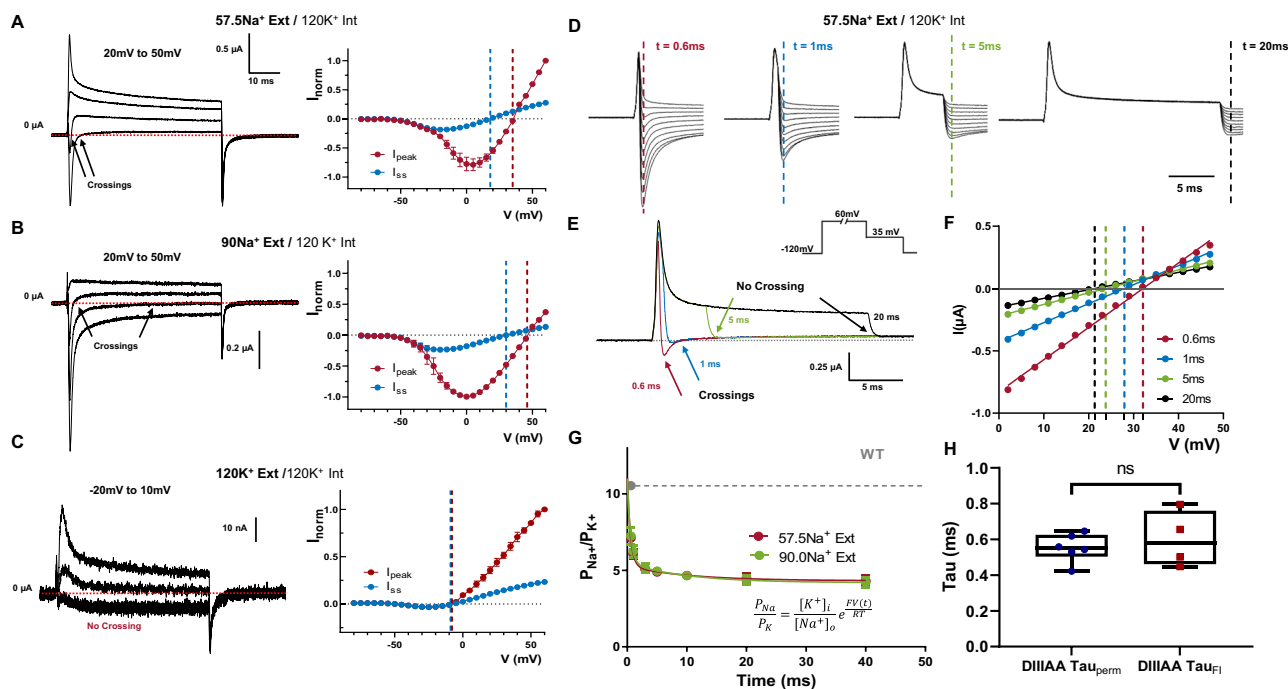
Fig. 3 | Time-dependent selectivity changes in DIIIAA. DIIIAA currents at different voltages (range shown on top) using 57.5 mM external Na + (A), N = 3 , 90 mM external Na + (B), N = 3 or 120 mM external K + (C), N = 2 with 120 mM internal K + ; on the right I - V curves for the peak (red) and steady state (blue) current. The reversal potential for each component is denoted with a corresponding dashed line. D Instantaneous I - V protocol obtained at different times during depolarization. E Example of the changes in direction for the tail currents. F Example instantaneous I - V curves after a 0.6 (red), 1 (blue), 5 (green), and 20 (black) milliseconds depolarization times of a single oocyte. The solid lines represent a linear fit used to obtain the reversal potential (indicated by vertical dashed lines). G Relative Na + /K +
