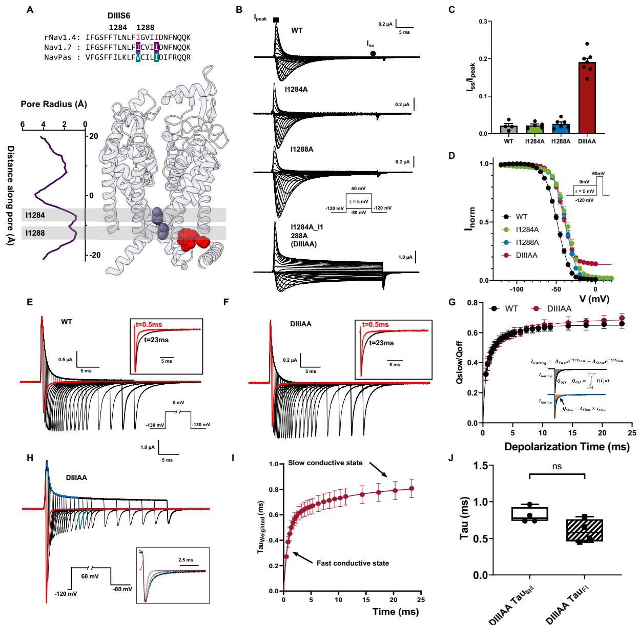
Fig. 2 | Double alanine mutation of the identified hydrophobic residues in DIII S6 creates a leaky inactivated state in Nav1.4. A Sequence alignment of DIII S6 showing identified residues (I1284 and I1288) and their positions in the Nav1.7 structure. B Representative ionic traces for the wild-type (WT), single (I1284A and I1288A), and double alanine (I1284A_I1288A, named DIIIAA) mutations of the identified residues on Nav1.4. The ionic conditions used were 57.5 mM Na + outside and 12 mM Na + inside. Inset shows the voltage protocol. WT, N = 4 ; I1284A N = 5 ; I1288A, N = 6 ; DIIIAA, N = 7 . C Ratio of steady state current ( I_{ss} , black circle) at the end of 30 ms depolarization over the peak current ( I_{peak} , black square) taken at +60 mV. D Voltage dependence of inactivation ( h -infinity curve) for WT (black), I1284A (green), I1288A (blue), and DIIIAA (red). Inset shows the voltage protocol. The lines represent the fit to a two-state model (Eq. 1). WT, N = 8 ; I1284A, N = 6 ; I1288A, N = 6 ; DIIIAA, N = 4 . E , F Representative traces of gating current for WT ( E ) and DIIIAA ( F ). Inset shows the voltage protocol. The black square top inset shows the comparison of the normalized gating current after 0.5 ms and 23 ms
