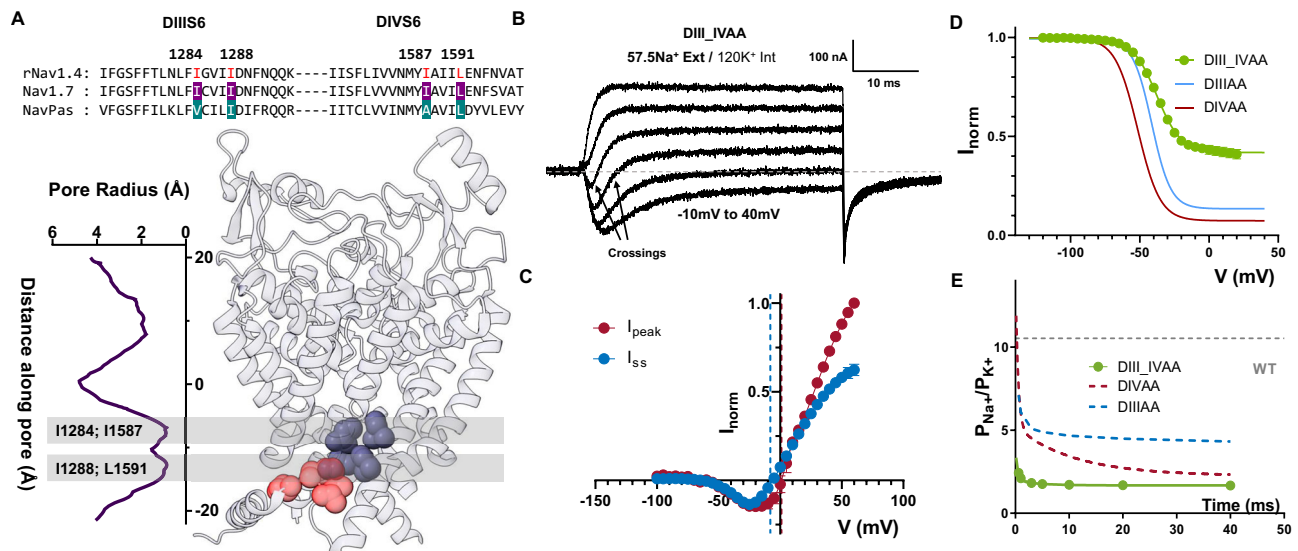
Fig. 6 | Quadruple alanine mutation of the identified residues in DIII & DIV S6 enhanced the phenotype seen in DIIIAA and DIVAA. A Sequence alignment of DIII, DIV S6 showing identified residues (highlighted in red) and their positions in the Nav1.7 structure. B Representative current traces elicited at different voltages (-10 to 40 mV) for the quadruple alanine mutation (I1284A_I1288A_I1587A_I1591A, DIII_IVAA) in 57.5 mM external Na + and 120 mM internal K + . C I-V curves for the peak (red, N = 4) and steady state (blue, N = 4) current. The reversal potential for each
