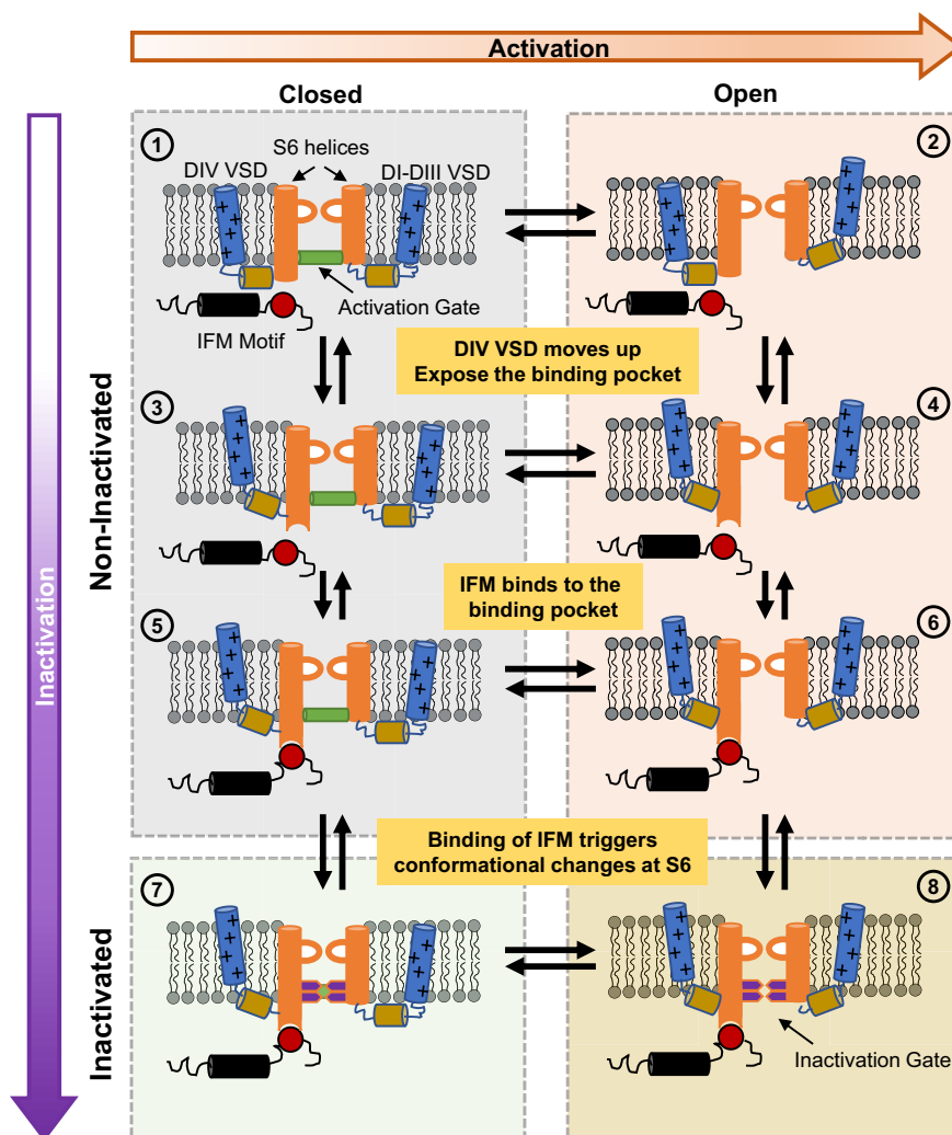
Fig. 8 | A general model for fast inactivation from open or closed states. For simplicity, the multi-step activation is shown as a single transition between the last closed state and the open state in the horizontal direction (rightward), and vertical transitions represent the fast inactivation pathway (downward). ① represents the Nav channel in the last closed state. ② represents the channel with the VSD of DI–DIII in the active (up) position, DIV VSD in the resting (down) position, and a conducting pore: an open channel. Transitions from ① to ③ and ② to ④ occur when DIV VSD
