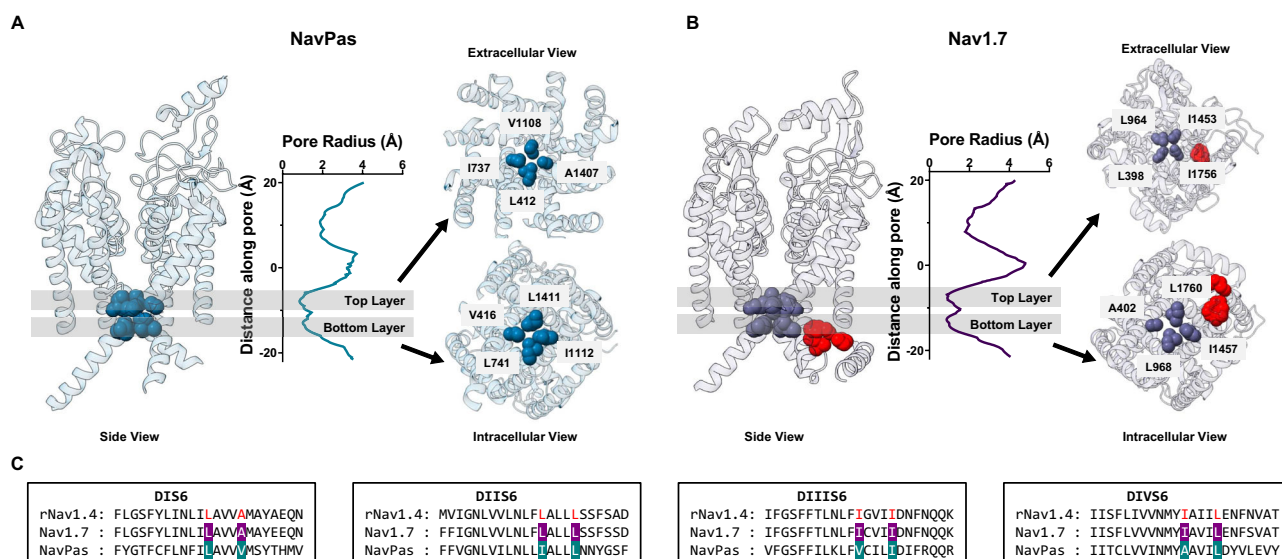
Fig. 1 | Pore radius profiles of NavPas and Nav1.7 show two layers of hydrophobic barriers. A Structure of NavPas (PDB:6A95 30 ). B Structure of Nav1.7 M11 (PDB:7XVF 28 ). The IFM motif is highlighted in red. The pore radius was calculated using HOLE 31 . NavPas and Nav1.7 structures show similar pore profiles at the bottom of S6, where two layers of the hydrophobic barrier are identified (shadowed regions). Identified top (extracellular view) and bottom (intracellular view) hydrophobic layers in NavPas and Nav1.7 are shown. In NavPas, the top layer is formed by
