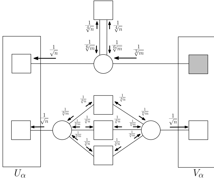
Figure 4.6: Allocation of \frac{1}{\sqrt{n}} from each edge to vertices. S consists of the gray square. Observe that every circle receives a factor of at least \frac{1}{\sqrt{m}} and every square not in S receives a factor of at least \frac{1}{\sqrt{n}} .
