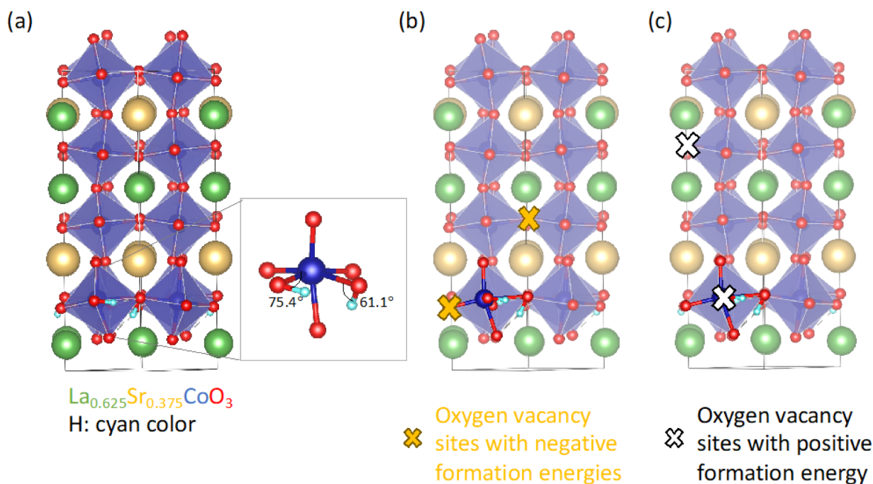
Figure 3. (a) Hydrogen configuration with the lowest formation energy ( \Delta E_{\text{HH}} ), where the \text{H}_2 molecules decompose and form two neighboring -\text{OH} bonds. The inset figure shows details of the -\text{OH} bonding structure, with the \text{Co}-\text{OH} bond angle marked in the figure. (b) Oxygen vacancy sites with negative oxygen vacancy formation energies ( \Delta E_{\text{VO}} ), which are close to -\text{OH} bonds. (c) Oxygen vacancy sites with positive oxygen vacancy formation energy ( \Delta E_{\text{VO}} ), which are bonded to hydrogen.
