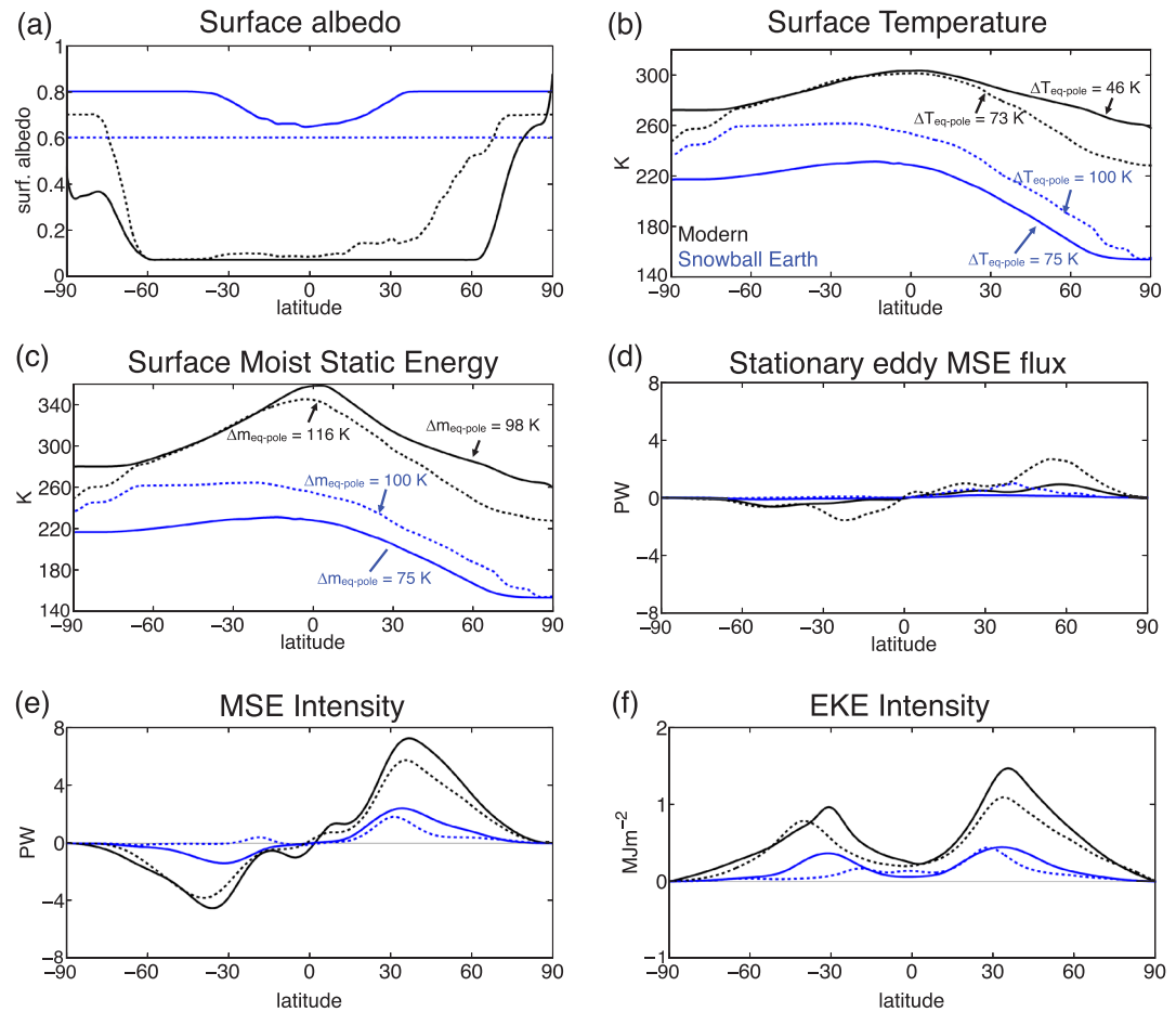
Figure 1. Northern Hemisphere wintertime (a) surface albedo, (b) surface temperature, (c) surface MSE (divided by specific heat at constant pressure), (d) stationary eddy MSE flux, and storm track intensity defined by vertically integrated (e) transient eddy MSE flux and (f) EKE for AGCM (dashed) and AQUA (solid) modern (black) and Snowball Earth (blue) simulations.
