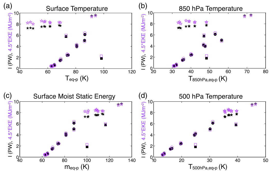
Figure 4. Storm track intensity versus equator minus pole (a) surface (2 m) temperature, (b) 850 hPa temperature, (c) surface (2 m) MSE, and (d) 500 hPa temperature across a range of simulated climates between Snowball Earth and modern. MSE and EKE (multiplied by 4.5) intensity indicated by black and purple symbols, respectively. AGCM simulations shown by squares and AQUA simulations shown by stars and circles with circles denoting Snowball Earth simulations.
