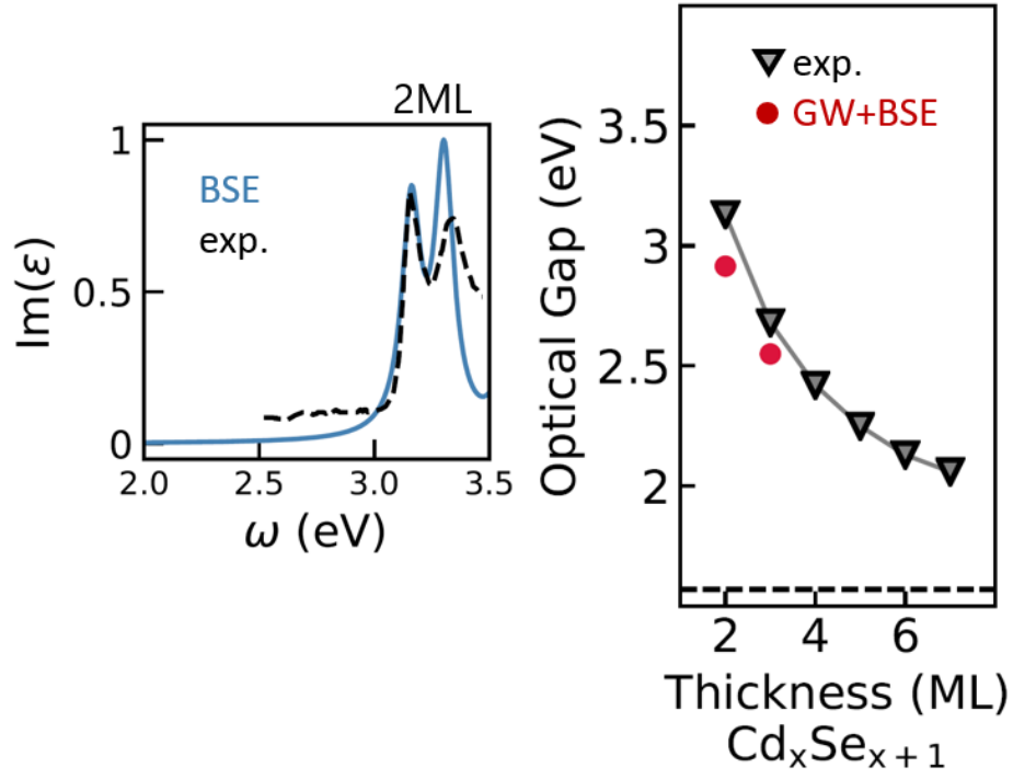
Figure 5.13: a) BSE spectrum of 2ML CdSe calculated using 15x15x1 k-point sampling compared to experimental data from [83]. BSE spectrum is plotted with a Lorentzian broadening of 0.05 eV. b) Optical band gaps using G_0W_0 fundamental gaps and E_b calculated from BSE
