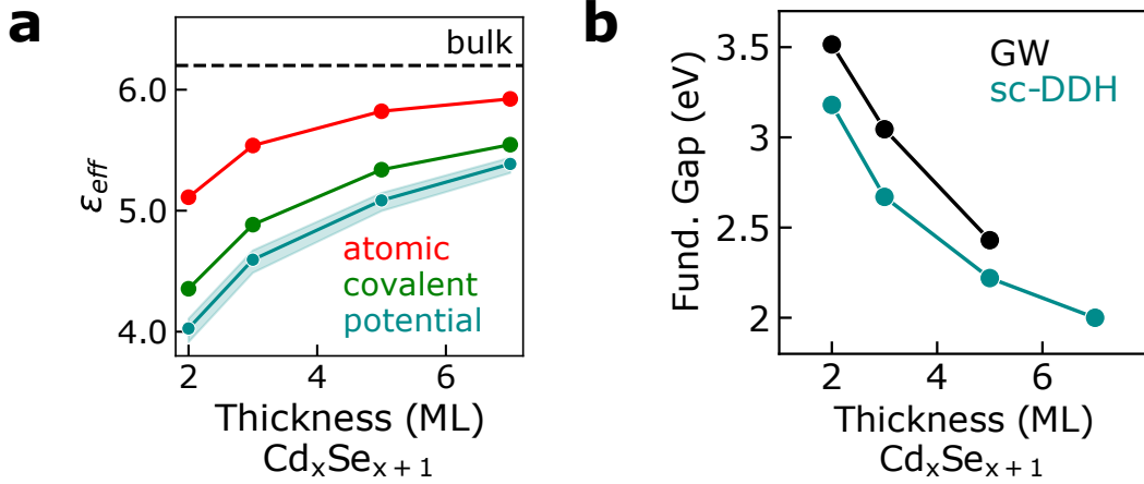
Figure 5.12: a) Effective dielectric constants of the NPLs calculated using three definitions of the NPL thickness: the atom-to-atom distance (red), the covalent radii (green) and the electrostatic potential (teal). Error bars on the teal curve represent the maximum and minimum thicknesses defined in Table 5.4.4. b) Fundamental band gaps calculated using sc-DDH compared to G_0W_0 .
