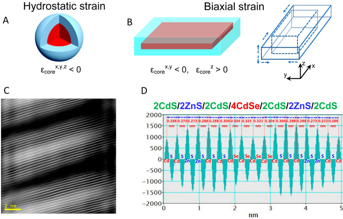
Figure 2.3: Figure and caption from Ref. [77]. Strain and tetragonal unit cell distortion in NPL heterostructures. (A, B) Comparison of strain caused by the lattice mismatch in core-shell nanostructures with spherical and NPL morphology. In a spherical QD, the core is hydrostatically strained while the NPL core is under biaxial strain: the lattice is compressed along the x and y coordinates and expanded along the z-axis, which is also the direction of strong quantum confinement. (C) HAADF-STEM image of 2CdS/2ZnS/2CdS/4CdSe/2CdS/2ZnS/2CdS and (D) the interplanar distances for this structure
