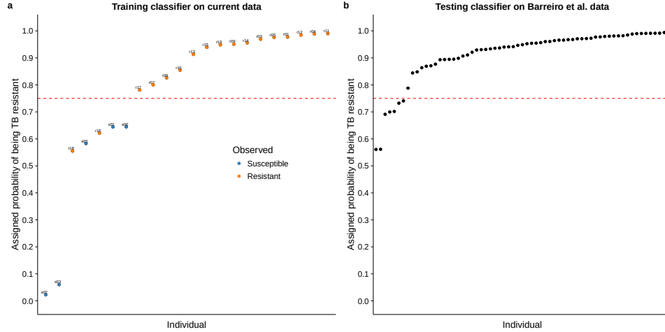
Figure 3.3: Classifying TB susceptible individuals using a support vector machine model. (a) The estimates of predicted probability of TB resistance from the leave-one-out-cross-validation for individuals in the current study. The blue circles represent individuals known to be susceptible to TB, and orange those resistant to TB. The horizontal dashed red line at a probability of 0.75 separates susceptible and resistant individuals. (b) The estimates of predicted probability of TB resistance from applying the classifier trained on the data from the current study to a test set of independently collected healthy individuals [17].
