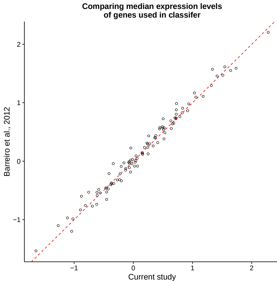
Figure 3.18: Comparing gene expression between the two studies. After normalization and batch-correction, the median expression levels of the 99 genes used in the classifier were similar between the samples in the current study and those in Barreiro et al., 2012 [17]. The dashed red line is the 1:1 line.
