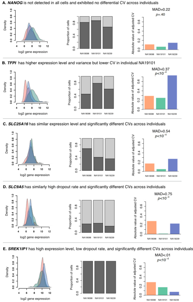
Figure 4.11: Inter-individual differences in regulatory noise. These 5 example genes illustrate various patterns of cell-to-cell gene expression variance. For each gene, the left panel shows the distribution of the \log_2 gene expression levels (considering only cells in which the gene is detected as expressed), the middle panel shows the proportion of cells in which the gene is detected as expressed (dark grey) and the dropout rate (light grey) for each individual, and the right panel shows the absolute value of adjusted CV for each individual, along with the corresponding gene-specific MAD (median of absolute deviation) value and P -value. The three colors in the upper and lower panel represent the individuals (NA19098 in red, NA19101 in green, and NA19239 in blue).
