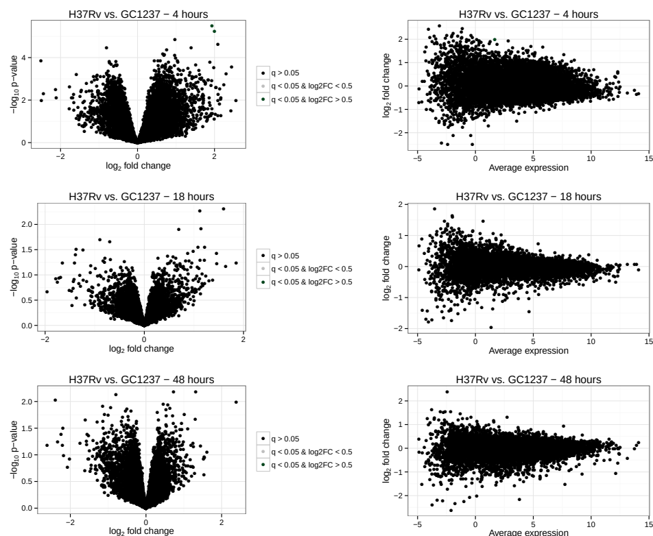
Figure 2.12: Little difference in transcriptional response to infections with different MTB strains. Few statistically significant differences were identified when explicitly testing gene expression levels post-infection with MTB H37Rv and MTB GC1237 at 4, 18, or 48 hours post-infection (top, middle, and bottom panels, respectively). The volcano plots (left) display the -\log_{10} transformed p-value versus the \log_2 fold change in expression level. The MA plots (right) display the \log_2 fold change in expression level versus the average expression level. Most of the genes are labeled black indicating that their FDR value is greater than 5%. Two genes (labeled green) at 4 hours post-infection had a q-value < 0.05 and \log_2 fold change greater than 0.5 (see Supplementary Table 2.9).
