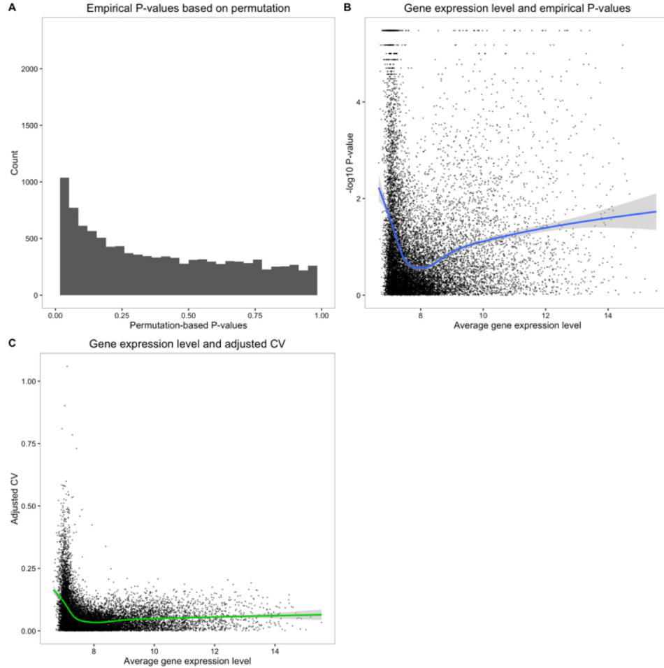
Figure 4.10: Permutation-based P -value. (A) Histogram of empirical P -values based on 300,000 permutations. (B) -\log_{10} empirical P -values are plotted against average gene expression levels. Blue line indicates the fitted relationship between -\log_{10} P -values and average \log_2 gene expression levels of cells that were detected as expressed, using locally weighted scatterplot smoothing (LOESS). (C) Median of Absolute Deviation (MAD) of genes versus average gene expression levels. Green line indicates the fitted relationship (LOESS) between the MAD values and average \log_2 gene expression levels of cells in which the gene was detected as expressed.
