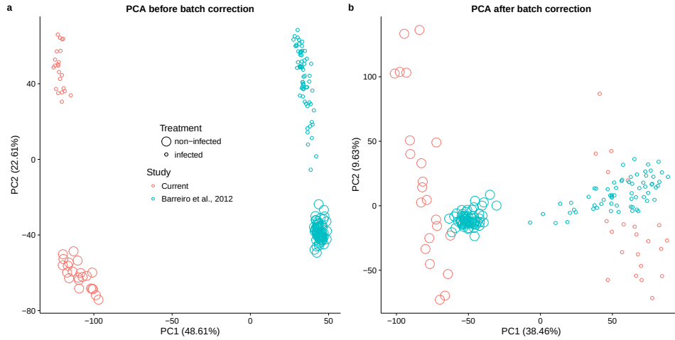
Figure 3.14: Principal components analysis (PCA) of combined data sets. (a) PC1 versus PC2 of the combined data set of the RNA-seq data from the current study (red) and the microarray data from Barreiro et al., 2012 [17] (blue). The large circles are non-infected samples, and the small circles are infected samples. The value in parentheses is the percentage of the total variation accounted for by that PC. (b) The same data after regressing the original PC1 in (a).
