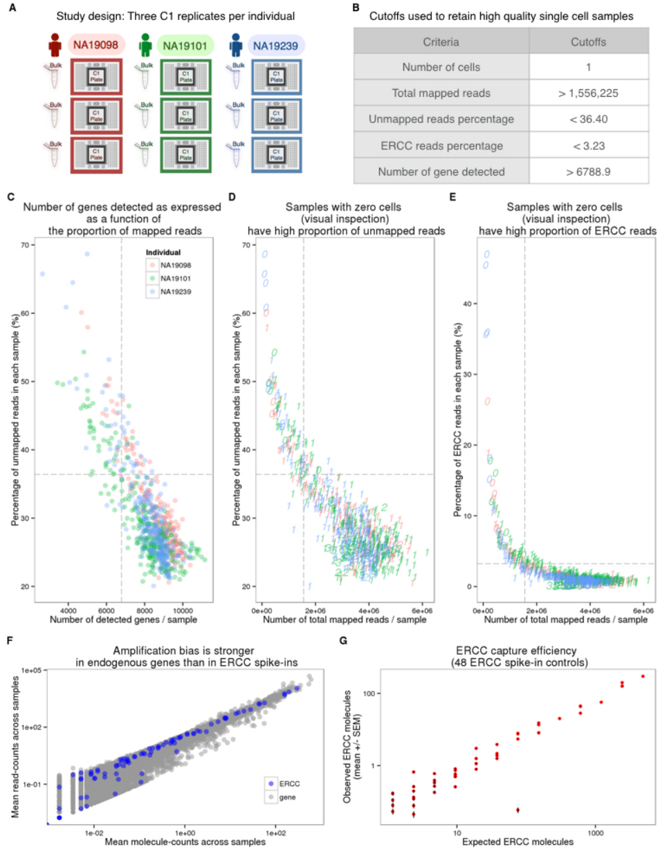
Figure 4.1: Experimental design and quality control of scRNA-seq. (A) Three C1 96 well-integrated fluidic circuit (IFC) replicates were collected from each of the three Yoruba individuals. A bulk sample was included in each batch. (B) Summary of the cutoffs used to remove data from low quality cells that might be ruptured or dead (See Supplementary Fig. 4.6 for details). (C-E) To assess the quality of the scRNA-seq data, the capture efficiency of cells and the faithfulness of mRNA fraction amplification were determined based on the proportion of unmapped reads, the number of detected genes, the numbers of total mapped reads, and the proportion of ERCC spike-in reads across cells. The dash lines indicate the cutoffs summarized in panel (B). The three colors represent the three individuals (NA19098 in red, NA19101 in green, and NA19239 in blue), and the numbers indicate the cell numbers observed in each capture site on C1 plate.
