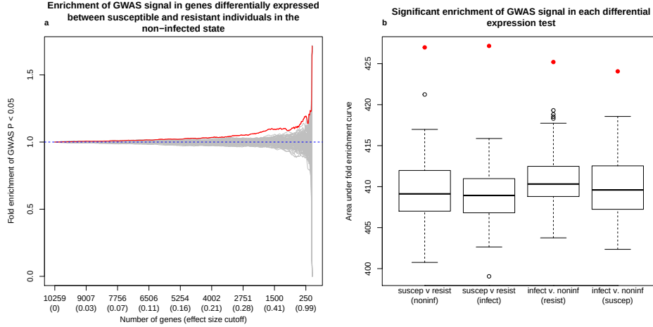
Figure 3.2: Comparison of differential expression and The Gambia GWAS results.
