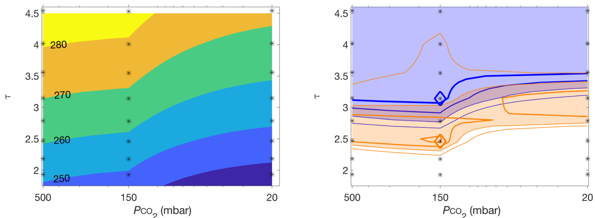
Fig. 5. Best-fit Mars climate versus time. (Left) Global annual average temperature (K) as a function of P_{\text{CO}_2} and of gray gas column optical depth, \tau . Black asterisks correspond to inputs to individual GCMs, and values between the asterisks are interpolated. Obliquity = 45°. (Right) Goodness of fit of model to data as a function of P_{\text{CO}_2} and of gray gas column optical depth, \tau . Blue shaded region corresponds to relatively good fit to >3.6-Ga data, and orange shaded region corresponds to relatively good fit to <3.6-Ga data. The blue diamond is the best-fitting GCM run for >3.6-Ga data, and the orange diamond is the best-fitting GCM run for <3.6-Ga data. Metric is ROC AUC; contours correspond to 0.5, 0.55, 0.6, and 0.65 (thicker lines correspond to better fit). Asterisks correspond to inputs to individual GCMs, and values between the dots are interpolated. Figures S14 and S15 give more details and sensitivity tests.
