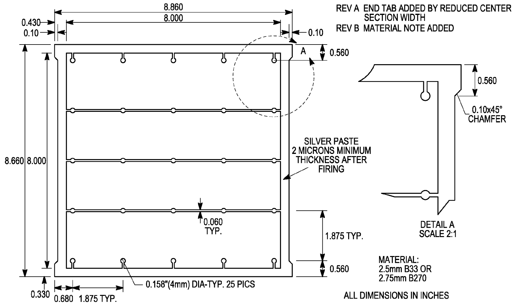
WINDOW HIGH VOLTAGE DISTRIBUTION PATTERN
