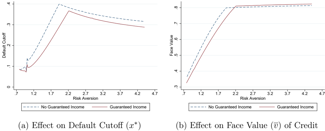
Figure C.20: Risk Aversion and Effect on Default Cutoff and Face Value
