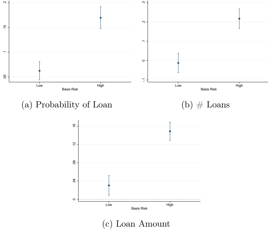
Figure A.9: Heterogeneous Treatment Effect on Borrowings by Basis Risk
