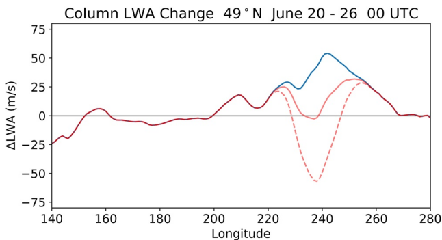
Figure 5. Blue: observed change in column local wave activity (LWA) between 20 and 26 June 2021 00 UTC at 49°N. Solid-red: reconstructed change in column LWA with 70 percent of positive diabatic forcing in 200–220°E during 22–24 June. Dashed-red: Same as solid-red but with positive diabatic forcing completely suppressed in 200–220°E during 22–24 June.
