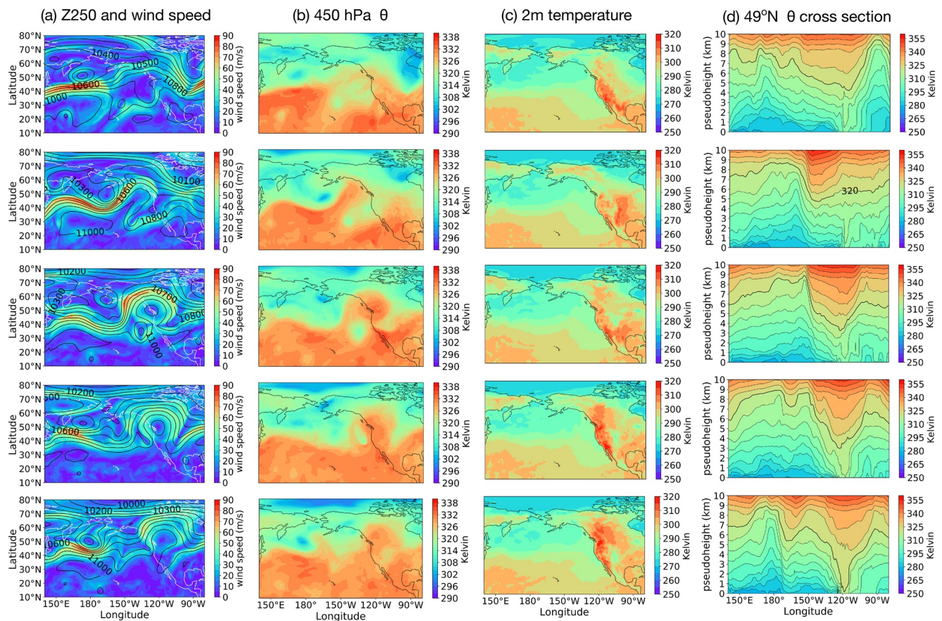
Figure 1. Circulation and temperature over North Pacific and North America 22–30 June 2021. Rows are, from top to bottom, 22, 24, 26, 28, 30 June at 00 UTC. Column (a) 250 hPa geopotential height (contours in meters) and wind speed. Column (b) 450 hPa potential temperature. Column (c) 2-m temperature. Column (d) vertical cross sections of potential temperature at 49°N (contour interval = 5 K). The 320-K isentrope is highlighted. The vertical axis is pressure pseudoheight with H = 8 km (450 hPa = 6.4 km). Data source: ERA5 (Figures 1–4).
