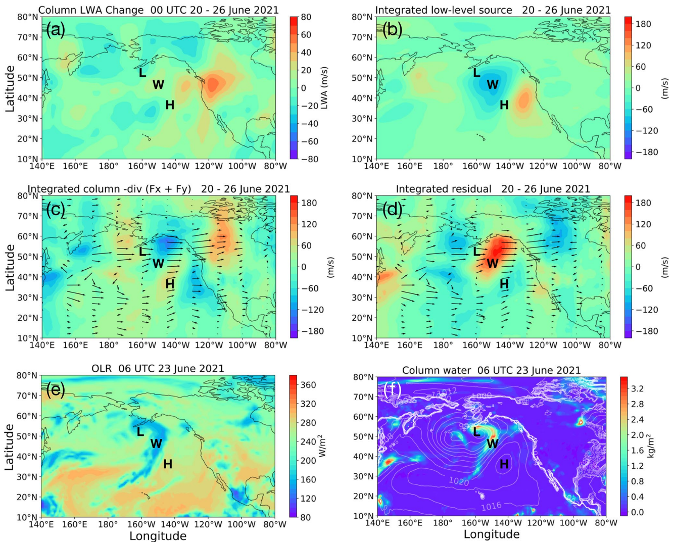
Figure 3. (a) Map of the LHS of Equation 3 integrated from 20–26 June 2021 00 UTC. (b) Same as (a) but for Term (III). (c) Same as (b) but for Terms (I)+(II). See Figure S1 in Supporting Information S1 for Term (II). (d) Same as (c) but for Term (IV). Arrows in (c) and (d) indicate the change in the 6-day average \langle\langle F_\lambda \rangle\rangle from the previous 6 days (14–20 June). The longest arrow is 40 \text{ m}^2\text{s}^{-2} . For (a)–(d), a 10^\circ running mean is applied in the longitude to suppress noise. Note the different color scale for (a). (e) Outgoing longwave radiation at the top of the atmosphere at 06 UTC 23 June 2021. (f) Same as (e) but for column water (excluding vapor) and sea level pressure (in hPa). Labels L, H, and W indicate, respectively, the locations of surface low pressure, high pressure, and warm conveyor belt at 06 UTC 23 June 2021 (panel f).
