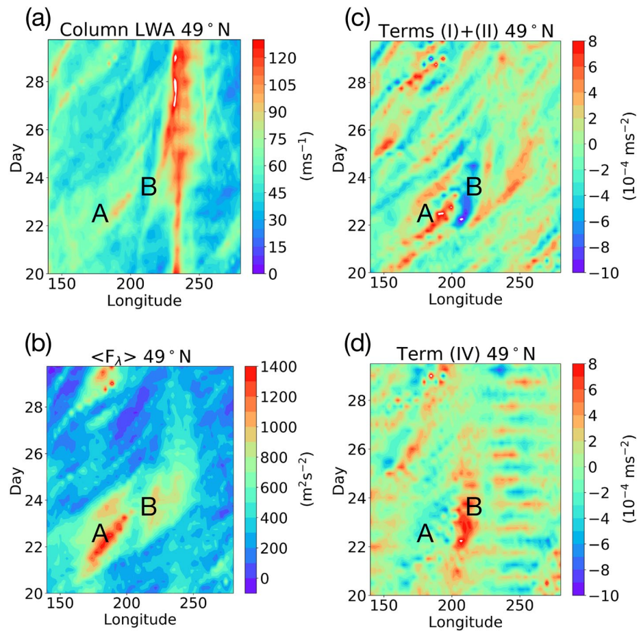
Figure 4. (a) Hovmöller diagram of column local wave activity at 49°N for 20–30 June 2021 00 UTC. (b) Same as (a) but for the column mean zonal wave activity flux \langle F_\lambda \rangle . (c) Same as (b) but for Terms (I)+(II) in Equation 3. (d) Same as (c) but for Term (IV). A 10° running mean is applied in longitude for (c) and (d). The regularly spaced zonal striping in 225–270°E in (d) reflects the diurnal cycle in land-surface heating. Labels A and B indicate enhanced downstream transmission of wave activity and a wave activity source associated with cyclogenesis, respectively.
