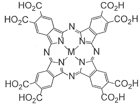
Phthalocyanine-octacarboxylic acid
