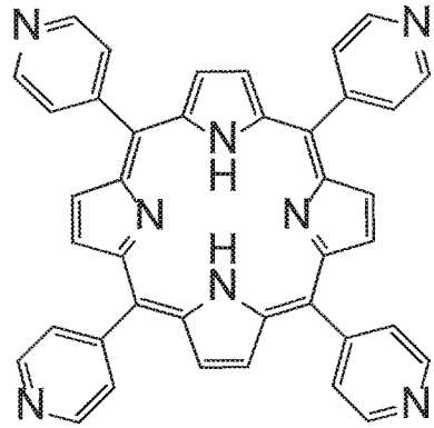
5,10,15,20-tetra(p-pyridyl)porphyrin
