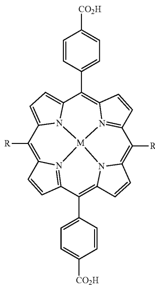
Scheme 2. Exemplary Metal Complex DBP, DBC, and DBBC ligands.
