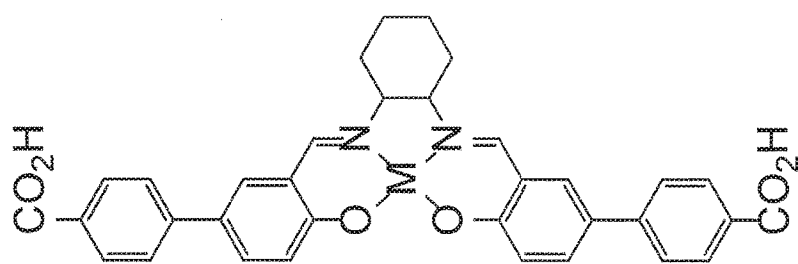
disalicylidene-1,2-cyclohexyldenediamine complex
