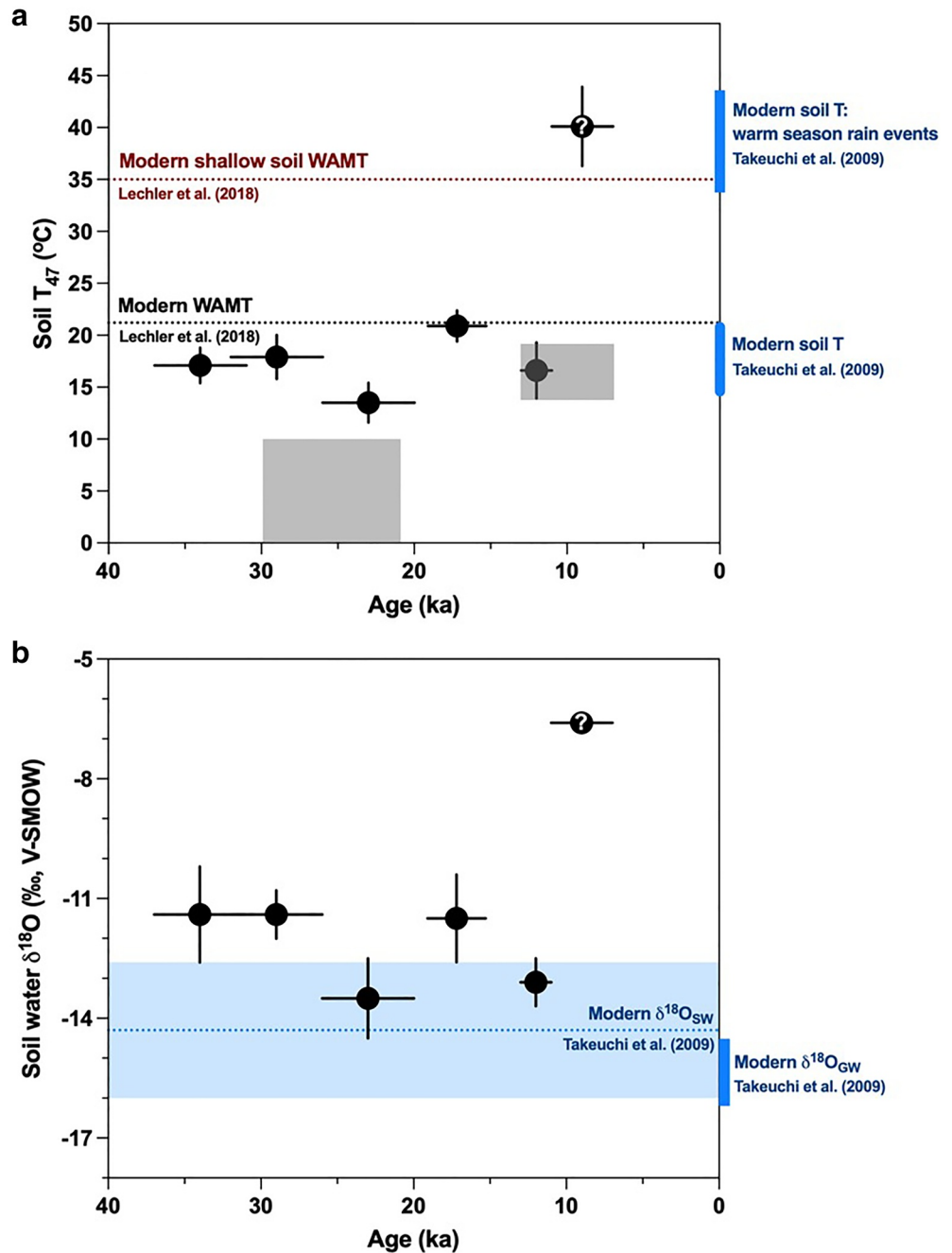
Figure 3. Estimates of soil carbonate formation temperatures from clumped isotopes (Soil T_{\Delta_{47}} ) and water \delta^{18}\text{O} over the past 40 ka. (a) Black circles indicate soil carbonate formation temperatures results from this work calculated using our measurements of T_{\Delta_{47}} and the temperature calibration from Anderson et al. (2021). Black symbol with question mark indicates data from samples that formed during the Holocene Climatic Optimum, that could record formation during conditions similar to modern warm season rain events in shallow soils, after Lechler et al. (2018), or could be impacted by radiative heating effects. Shaded gray boxes indicate temperatures reconstructed by Lechler et al. (2018). Blue vertical bars on the right indicate modern soil temperatures associated with carbonate precipitation derived from modern Palouse loess soil water samples and soil carbonates from Takeuchi et al. (2009). Black dotted line indicates modern warm month mean temperatures, while blue dotted line indicates temperatures during modern warm season rain events, and red dotted line indicates modern shallow soil warm month mean temperatures, after Lechler et al. (2018). (b) Black circles indicate results calculated using the carbonate-water \delta^{18}\text{O} calibration of Kim and O'Neil (1997). Blue dotted line with blue shading indicates modern soil water \delta^{18}\text{O} and groundwater \delta^{18}\text{O} from Takeuchi et al. (2009), respectively. Blue vertical bar on the right indicates modern groundwater \delta^{18}\text{O} from Takeuchi et al. (2009).
