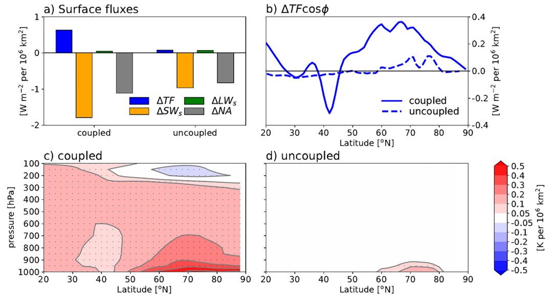
Figure 2. Response of summertime (a) high-latitude ( 50^{\circ}\text{N} – 90^{\circ}\text{N} ) surface energy flux (defined as positive upward), (b) zonal-mean surface turbulent flux (multiplied by the cosine of latitude), and (c, d) zonal-mean temperature to Arctic sea ice loss in the coupled and uncoupled climate model simulations. In (c, d), stipples indicate where all models agree in the sign of the response.
