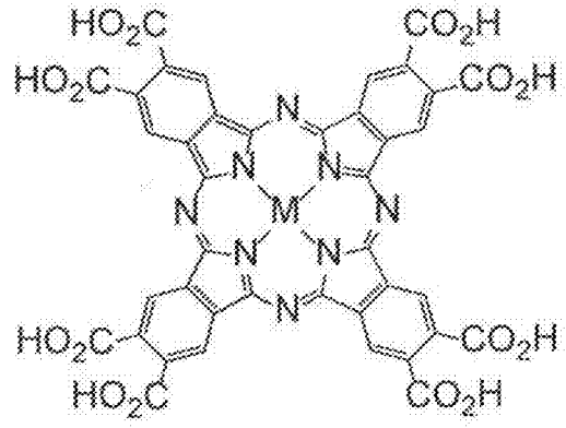
Phthalocyanine-octacarboxylic acid
