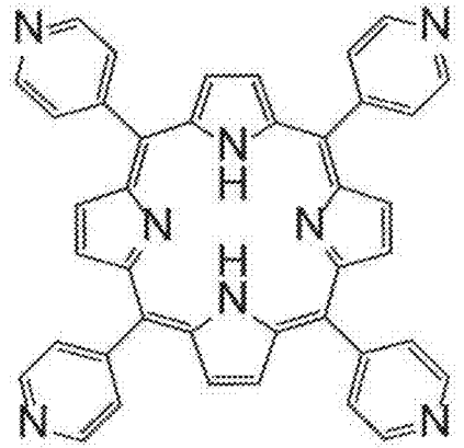
5,10,15,20-tetra(p-pyridyl)porphyrin
