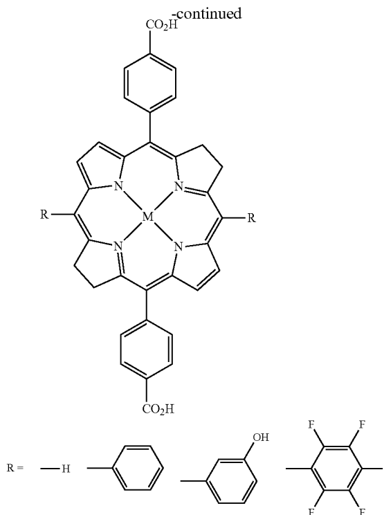
Scheme 2. Exemplary Metal Complex DBP, DBC, and DBCC ligands.
