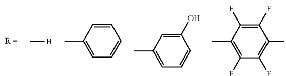
DBP, DBC, DBBC ligands and their derivatives
