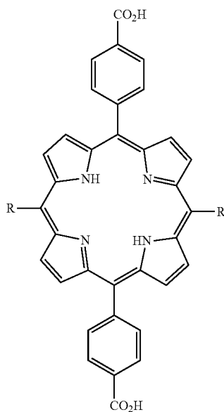
Scheme 1. Exemplary DBP, DBC, and DBCC ligands.
