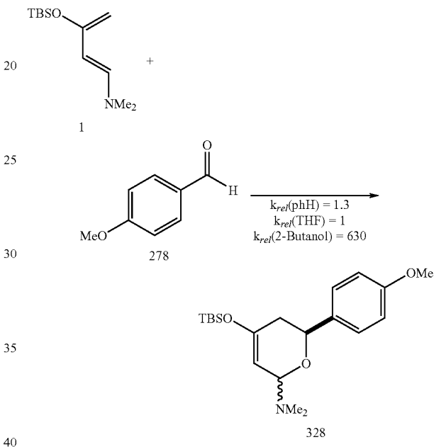
Scheme 8 - Hydrogen Bond Activation by 2-Butanol
