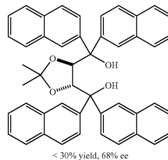
Scheme 10 - Results with Naphthyl-TADDOLs
