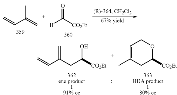
Scheme 7 - Chemoselective HDA Reactions Catalyzed by Metal Catalyst
