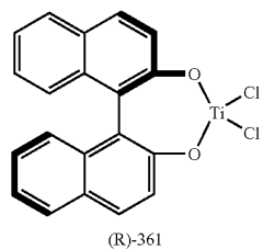
Scheme 7 - Chemoselective HDA Reactions Catalyzed by Metal Catalyst
