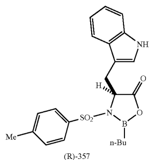
Scheme 6 - HDA and Ene Reactions Catalyzed by Metal Catalysts
