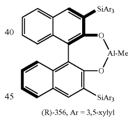
Scheme 5 - HDA Reactions Catalyzed by Tryptophan-derived Lewis Acid Catalyst
