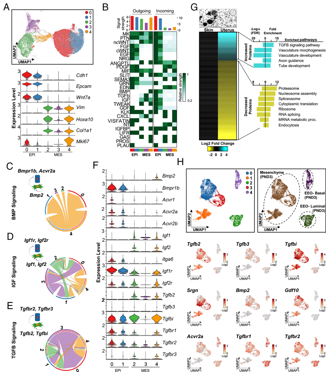
Fig. 4. Epithelial and mesenchymal crosstalk governs neonatal uterine development. (A) UMAP plot of integrated scRNA-seq analysis of mesenchyme (35) and epithelium (27) from neonatal uteri (Top). Violin plots represent annotation of cell types based on known marker genes (Bottom). (B) Heatmap comparing the outgoing (Left) and incoming (Right) signaling patterns associated with both mesenchymal and epithelial cells. Shading denotes the relative signaling strength of a pathway across cell types. Colored bar plots on top depict the signaling strength of a particular cell cluster by summarizing all pathways in the heatmap. (C–E) Schematic of outgoing signaling from mesenchymal to epithelial cells for selected pathways. (F) Violin plots confirm the expression of ligands and receptors in each cell type. (G) Heatmap of differentially abundant proteins determined by mass spectrometry analysis of uterine mesenchyme and skin fibroblast conditioned media. Representative bright-field images illustrating the impact of skin fibroblast and uterine mesenchyme on EEO development (Top). (H) UMAP plots of integrated scRNA-seq analysis of uterine mesenchyme (35) and EEO from PND3 females colored by cluster (Top Left) or cell type (Top Right). UMAPs in the bottom confirm the expression of ligands in the mesenchyme and receptors in EEOs.
