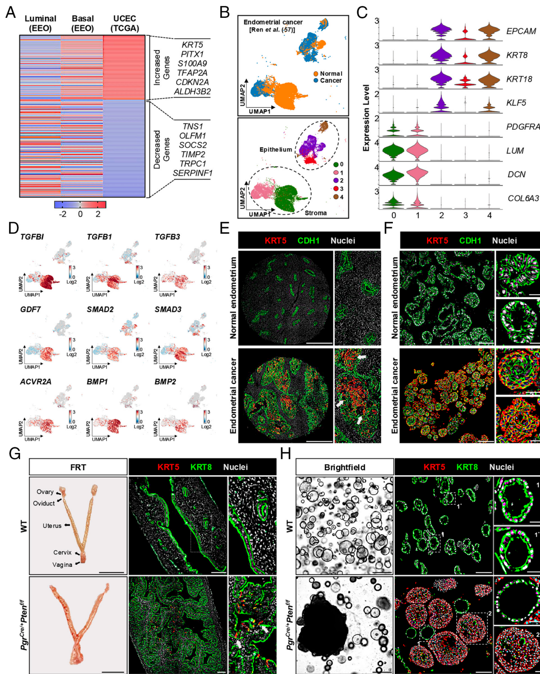
Fig. 5. Conserved epithelial dynamics between uterine development and disease. (A) Heatmap comparing the expression of luminal and basal EEO with human Uterine Corpus Endometrial Carcinoma (UCEC) from The Cancer Genome Atlas (TCGA) program. (B) UMAP of epithelial and stroma cells from human endometrial cancer (57) colored by disease state (Top) and cell type (Bottom). (C) Violin plots represent annotation of cell types based on known marker genes. (D) UMAP plots confirm the downregulation of TGFβ superfamily members in the stroma of endometrial cancer samples. (E and F) Immunofluorescent localization of KRT5 in endometrial biopsies (E, Scale bar, 500 μm) and patient-derived endometrial organoids (F, Scale bar, 100 μm; insets 20 μm). (G) Right panels: uteri of wildtype (WT) and Pgr Cre/+ Pten fl/fl mice. (Scale bar, 1 cm.) Left panels: immunofluorescent localization of KRT5 staining in uterine tissues. (Scale bar, 100 μm.) (H) Left panels: Representative bright-field images of EEOs established from WT and Pgr Cre/+ Pten fl/fl mice. (Scale bar, 500 μm.) Right panels: KRT5 staining is present in ML (2) but absent in SL (1) EEOs (Scale bar, 100 μm; insets 20 μm). White arrows indicate KRT5-positive epithelial cells in mouse and human uterine tissues.
