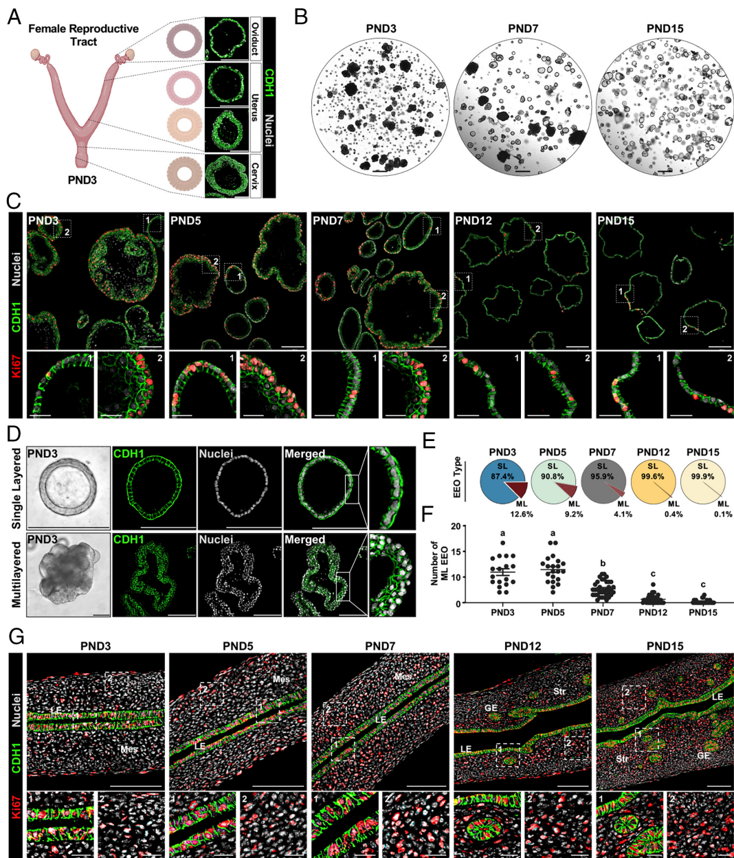
Fig. 1. Establishment and characterization of neonatal uterine organoids. (A) Illustration of oviductal, uterine, and cervical organoids established from postnatal day (PND) 3 female reproductive tracts (FRTs); Right panels: immunofluorescent localization of CDH1. (Scale bar, 100 \mu m.) (B) Representative low magnification bright-field images of endometrial epithelial organoids (EEO) established from PNDs 3, 7, and 15. (Scale bar, 100 \mu m.) (C) Immunofluorescent localization of Ki67 and CDH1 in EEO across developmental time points (Scale bar, 100 \mu m); insets represent single-layered (SL) (1) or multilayered (ML) (2) structures. (Scale bar, 20 \mu m.) (D) Representative images for SL and ML EEO. (Scale bar, 100 \mu m.) (E and F) Percentage of EEO type (E) and number of ML structures (F) across time points. All experiments were performed on passage 3 organoids ( n \geq 3 biological replicates per PND). Data are presented as mean \pm SEM. Solid dots represent technical replicates ( n \geq 3 biological replicates per PND) and letters indicate statistical differences between groups ( P < 0.001 ; ANOVA with the Bonferroni multiple-comparison test). (G) Immunofluorescent localization of Ki67 and CDH1 in neonatal uterine tissues (Scale bar, 100 \mu m); insets represent epithelium (1) or mesenchyme/stroma (2). (Scale bar, 20 \mu m.) GE, glandular epithelium; LE, luminal epithelium; Mes, mesenchyme; Str, Stroma.
