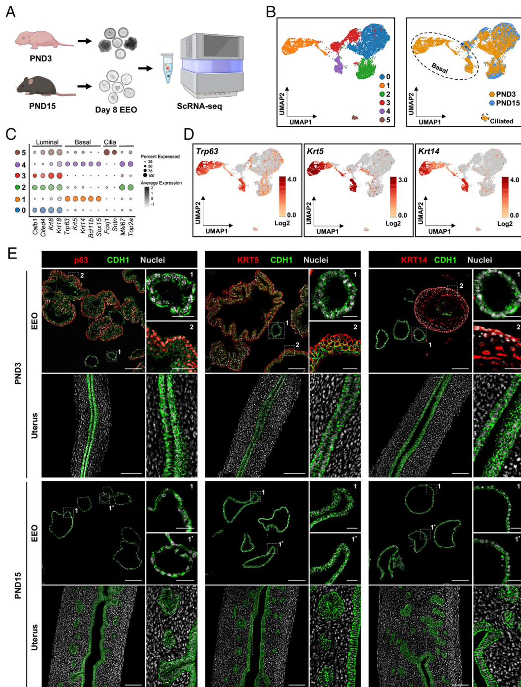
Fig. 2. Cellular heterogeneity of neonatal EEO. (A) Schematic illustration of experimental design. EEO established from PND 3 and 15 (n = 10 mice per PND) were collected after 8 d of culture and used for single cell RNA sequencing (scRNA-seq). (B) Uniform Manifold Approximation and Projection (UMAP) of cells colored by cell type (Left) or PND (Right); circled clusters represent basal and ciliated epithelium present only in the PND3 samples. (C) Dot plots represent the annotation of cell types based on known marker genes. (D) UMAPs of transcripts for the basal cell markers Trp63 , Krt5 , and Krt14 in the clusters unique to PND3 EEO. (E) Immunofluorescent localization of p63, KRT5, and KRT14 in EEO at passage 3 or uteri of mice at PND3 (Top) and 15 (Bottom). (Scale bar, 100 \mu m.) Basal cell markers were only expressed in ML (2) but not in SL (1, 1*) organoids.
