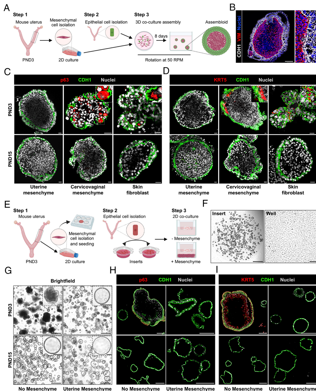
Fig. 3. Mesenchymal induction of uterine luminal epithelial fate. (A) Protocol for generating uterine assembloids. (B) Representative image of a uterine assembloid stained for epithelial (CDH1) and mesenchymal vimentin (VIM) cell markers. (Scale bar, 100 \mu m.) (C and D) Whole mount immunofluorescent localization for the basal cell markers p63 and KRT5 in assembloids. (Scale bar, 50 \mu m.) Assembloids were generated by combining uterine epithelium isolated from PND 3 (Top) or PND15 (Bottom) mice with PND3 uterine, cervicovaginal, or skin mesenchyme/fibroblast. (E) Experimental design for 2D coculture experiments. Epithelial cells were seeded in Cultrex on transwell inserts over PND3 uterine mesenchyme adhered to the bottom of 6-well plates and cultured for 20 d. (F) Representative bright-field images of EEO (Left; Scale bar, 500 \mu m) and mesenchymal cells (Right; Scale bar, 100 \mu m) in 2D coculture. (G) Representative bright-field images at day 20 of culture (Scale bar, 500 \mu m); insets show SL and ML organoids. (Scale bar, 100 \mu m.) (H and I) Immunofluorescent localization of p63 and KRT5 in organoids from PND3 (Top) and PND15 (Bottom) cocultures. (Scale bar, 100 \mu m.)
