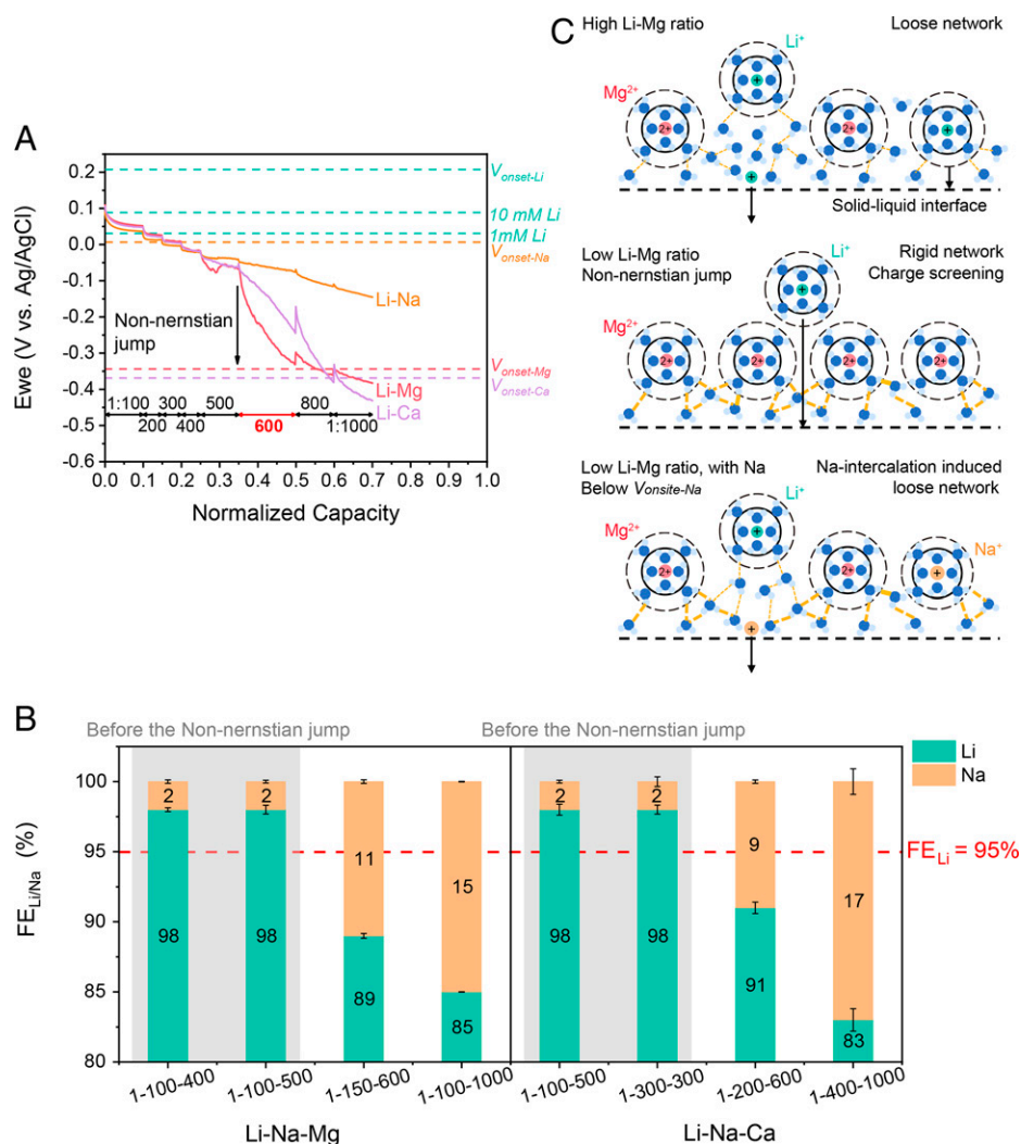
Fig. 4. Stepcon CP tests and host behavior in ternary solutions. (A) Stepcon CP tests in Li-Na/Mg/Ca binary systems with decreasing Li ratio from 1:100 to 1:1,000 ( [\text{Na}^+]/[\text{Mg}^{2+}]/[\text{Ca}^{2+}] is kept at 1 M; see Materials and Methods for more details; V_{\text{onset-Li/Na/Mg/Ca}} are acquired from the onset potential of the cathodic current peak during CV scan in Fig. 3A; 10 mM and 1 mM Li denote the Nernstian potential shift corrected by \text{Li}^+ concentration change). (B) Faraday efficiency of Li (green) or Na (orange) in Li-Na-Mg or Li-Na-Ca ternary systems ( [\text{Li}^+] is kept at 1 mM), calculated from ICP-MS recovery results. (C) Schematic showing different EDL structures induced by different compositions.
