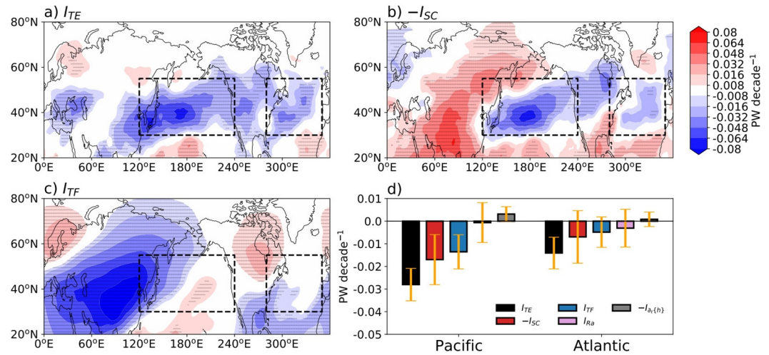
Figure 7. Spatial structure of JJA ensemble-mean trends from 1980 to 2020 of (a) storm track intensity ( I_{TE} ) and contributions from (b) stationary circulation ( -I_{SC} ) and (c) surface turbulent fluxes ( I_{TF} ) from the AER simulations. Statistically significant trends at the 95% confidence interval are stippled. The Pacific (30–55°N, 120–240°E) and Atlantic (30–55°N, 280–350°E) storm track domains are shown in black dashed box. (d) The ensemble-mean JJA storm track trends from 1980 to 2020 and their decomposition in the Pacific and Atlantic from the AER simulations. The 95% confidence intervals are shown with yellow errorbars.
