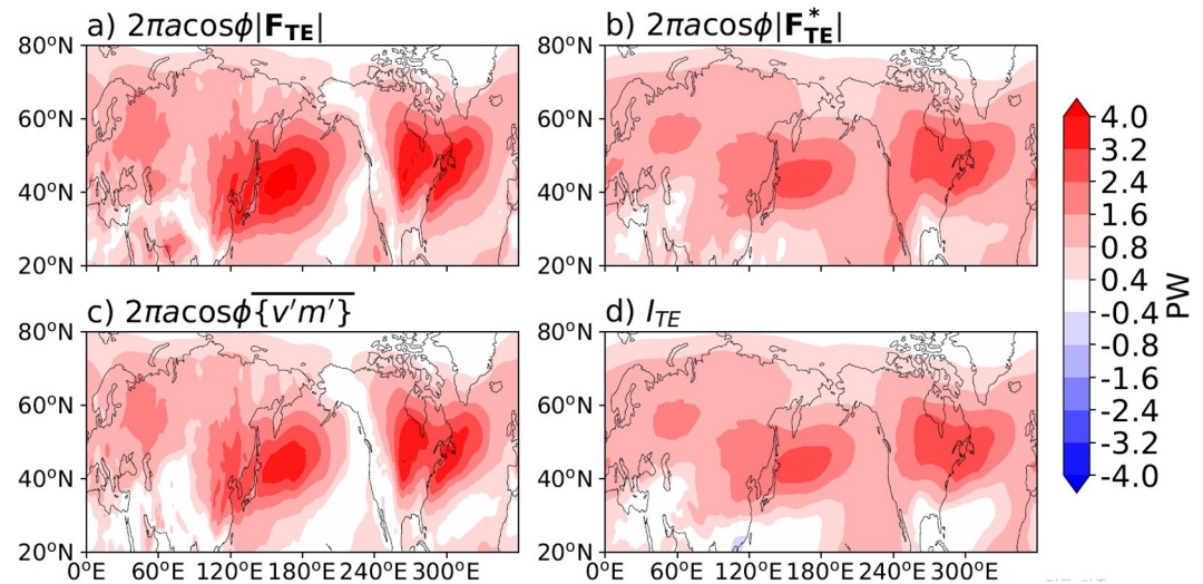
Figure A1. JJA climatology of (a) 2\pi\text{acos}\phi|\mathbf{F}_{TE}| , (b) 2\pi\text{acos}\phi|\mathbf{F}_{TE}^*| , (c) 2\pi\text{acos}\phi\overline{\{v'm'\}} , and (d) I_{TE} from ERA5 (1980–2020). In panels (a, b) absolute values of the flux vectors are shown, and (c, d) show the meridional component. I_{TE} is used as a definition of regional storm tracks.
